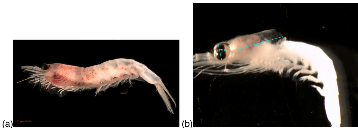
Fig. 3.6.1: Thysanopoda tricuspidata (a) and Nematoscellis atlantica (b)
