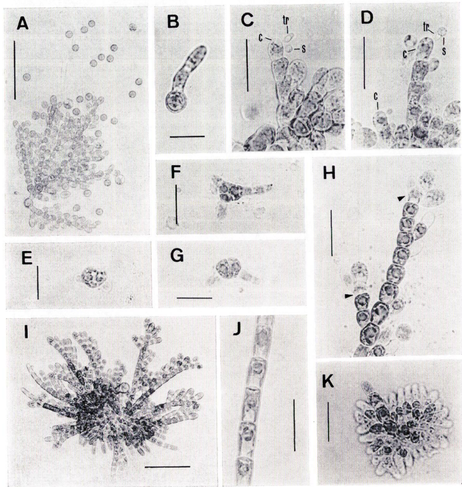
Fig. 5. Audouinella alariae in culture. A-D, H: gametophyte derived from monospore of gametophyte; A: gametophyte producing only monospores, B: germling of monospore, C, D: mature carpospore, H: mature carposporophyte on gametophyte (arrows). E-G, I-K: tetrasporophyte derived from carpospore; E-G, K: germination and development of carpospore, I: mature tetrasporophyte bearing tetrasporangia and monosporangia, J: showing plastid in vegetative cell.
