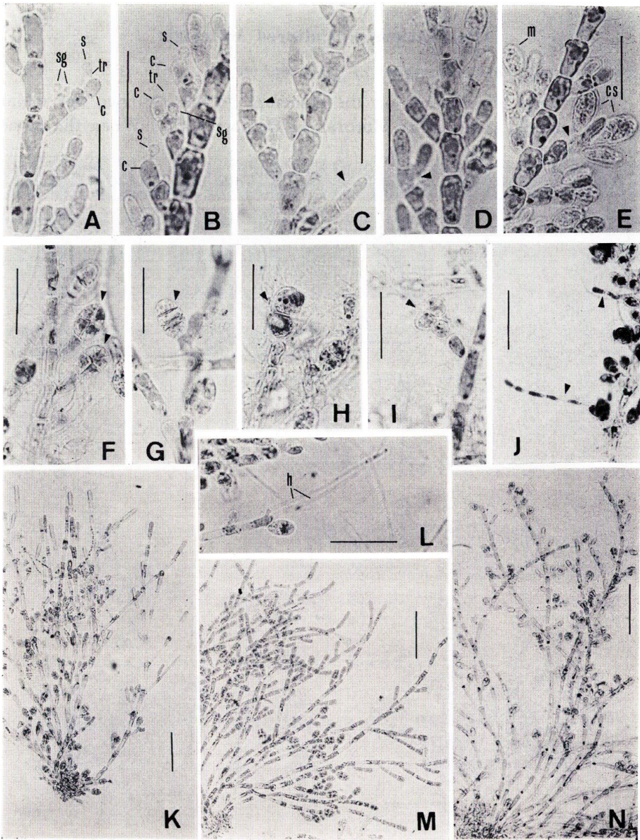
Fig. 4. Audouinella alariae in nature. A-E, J, L: gametophyte; A, B: spermatangia and carpospogonia developing terminally on short laterals, C, D: postfertilization development (arrows), showing elongation and transverse division of fertilized carpospogonia (C), and initial branching of carposporophyte (D), E: mature carposporophyte (arrow), J: in situ germination of monospores (arrows), L: terminal and subterminal hairs. F-I, K-N: tetrasporophyte; F: cruciately divided tetrasporangia (arrows), G: zonately divided tetrasporangium (arrow), H, I: aberrant sporangia (arrows), K, M, N: tetrasporophyte collected at Muroran in March (K), April (M) and May (N), note the basal (K), middle (M) and upper (N) regions of erect filaments where tetrasporangia occur. For abbreviation see Figs. 2 & 3. Scale bars: A-E=30 \mu m, F-I, L=40 \mu m, J=50 \mu m, K, M, N=100 \mu m.
