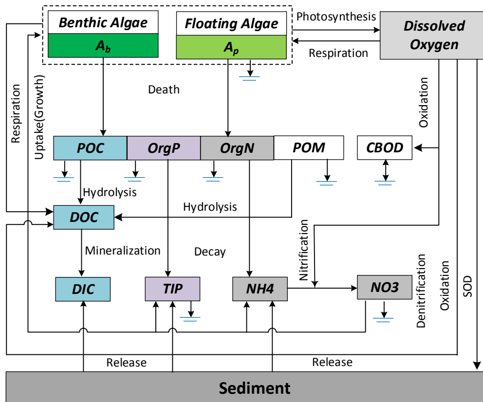
Figure 3. Water quality state variables and major processes modeled in NSMI.
