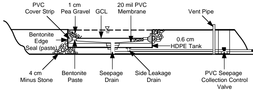
Figure 3. Details of the GCL test pans.
