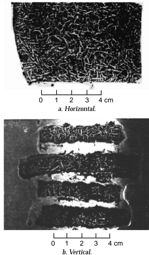
Figure 14. Thin sections of a frozen Bentomat GCL.
