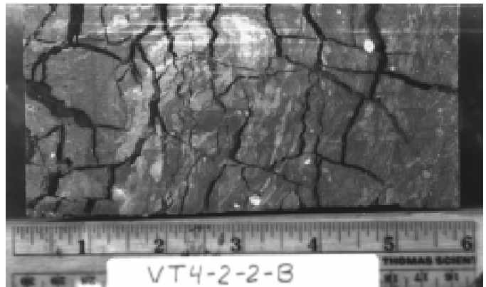
Figure 10. Vertical half section of Valley Trail frozen core. Note both ice-filled shrinkage cracks and ice lenses (black) surrounding clay aggregates (gray-white).
