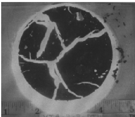
Figure 9. Thin section of a horizontal slice of frozen Valley Trail clay. Note thick ice features (white) in shrinkage cracks surrounding clay aggregates (black).
