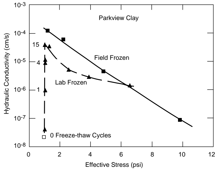
Figure 13. Impact of effective stress on the hydraulic conductivity of Parkview clay after freezing and thawing.
