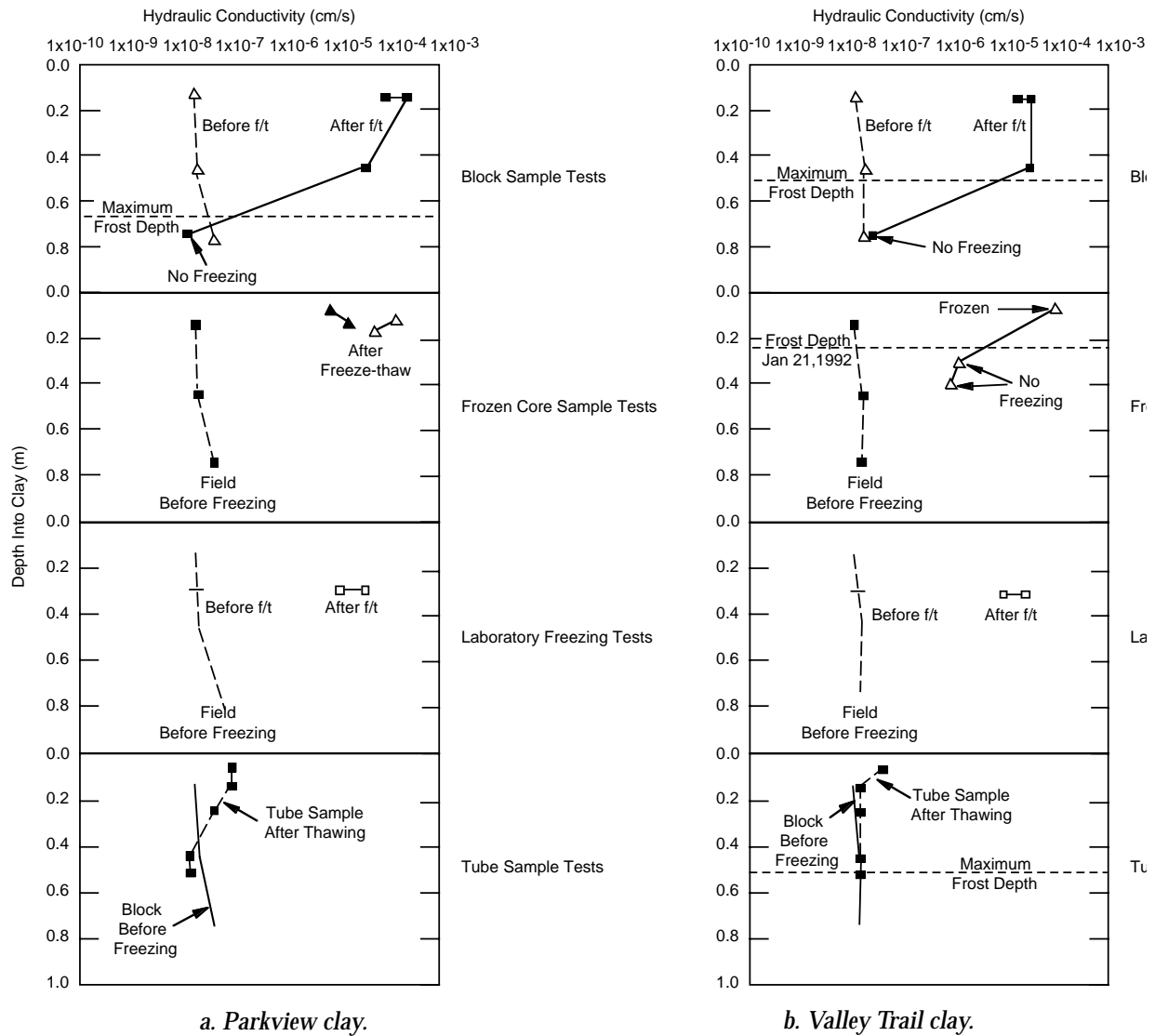
Figure 8. Summary of hydraulic conductivity test results.
