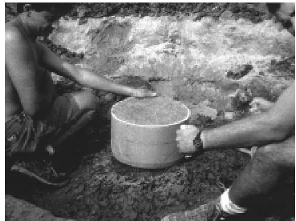
Figure 4. Taking a 12-in.- (30-cm-) diameter hydraulic conductivity test specimen from the field.
