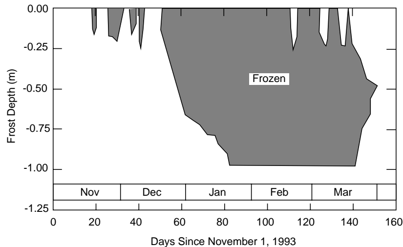
Figure 7. Example of the freeze and thaw depths during the winter of 1993–94.
