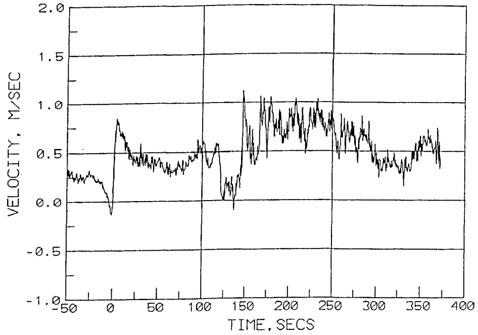
EXPERIMENT KV2323AT VELOCITY TIME HISTORY
