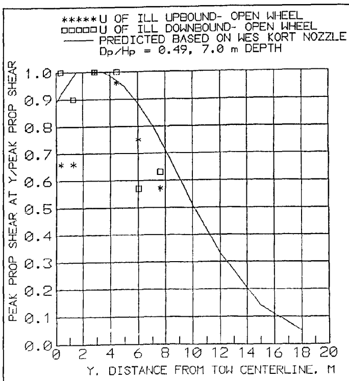
Figure 26. Lateral distribution of peak shear, open-wheel propellers, 7.8-m depth
