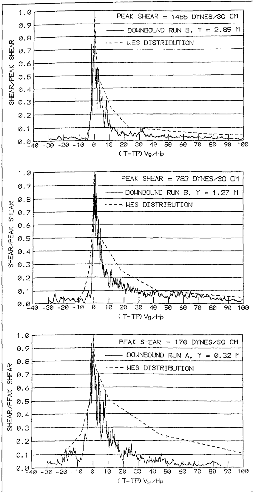
Figure 35. WES Kort nozzle distribution versus Garcia et al. (1998) open-wheel measurements
