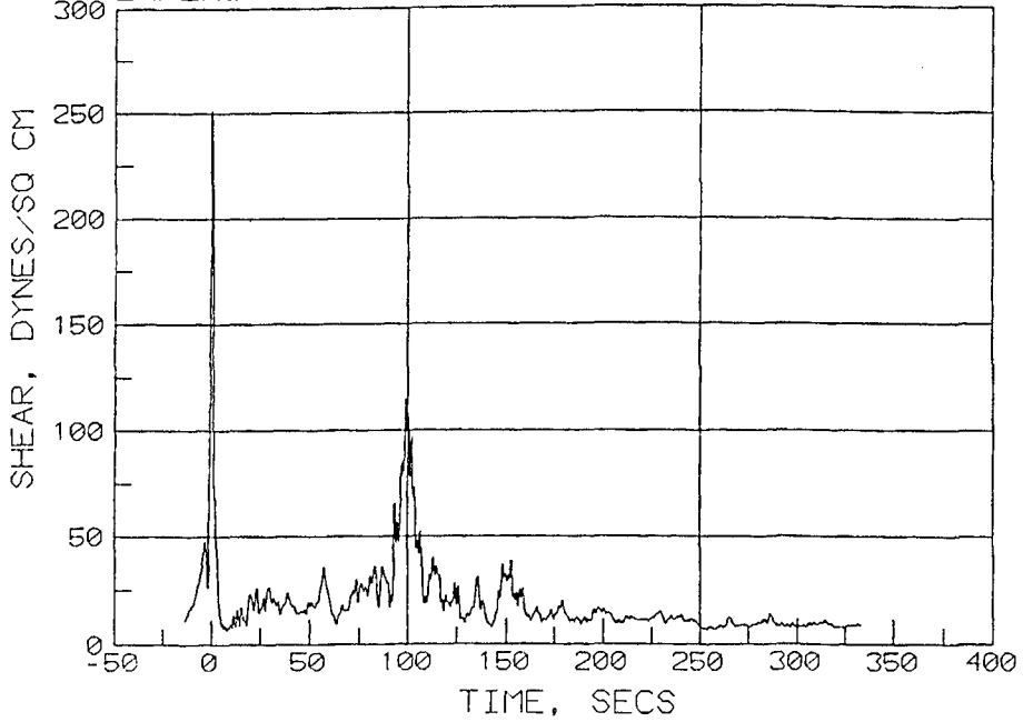
EXPERIMENT TU1524T8 MEASURED SHEAR
