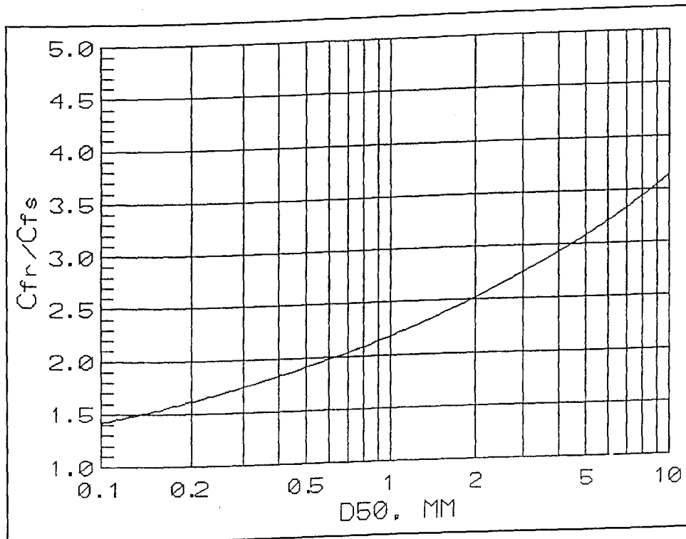
Figure 42. Local friction coefficient ratio versus D50
