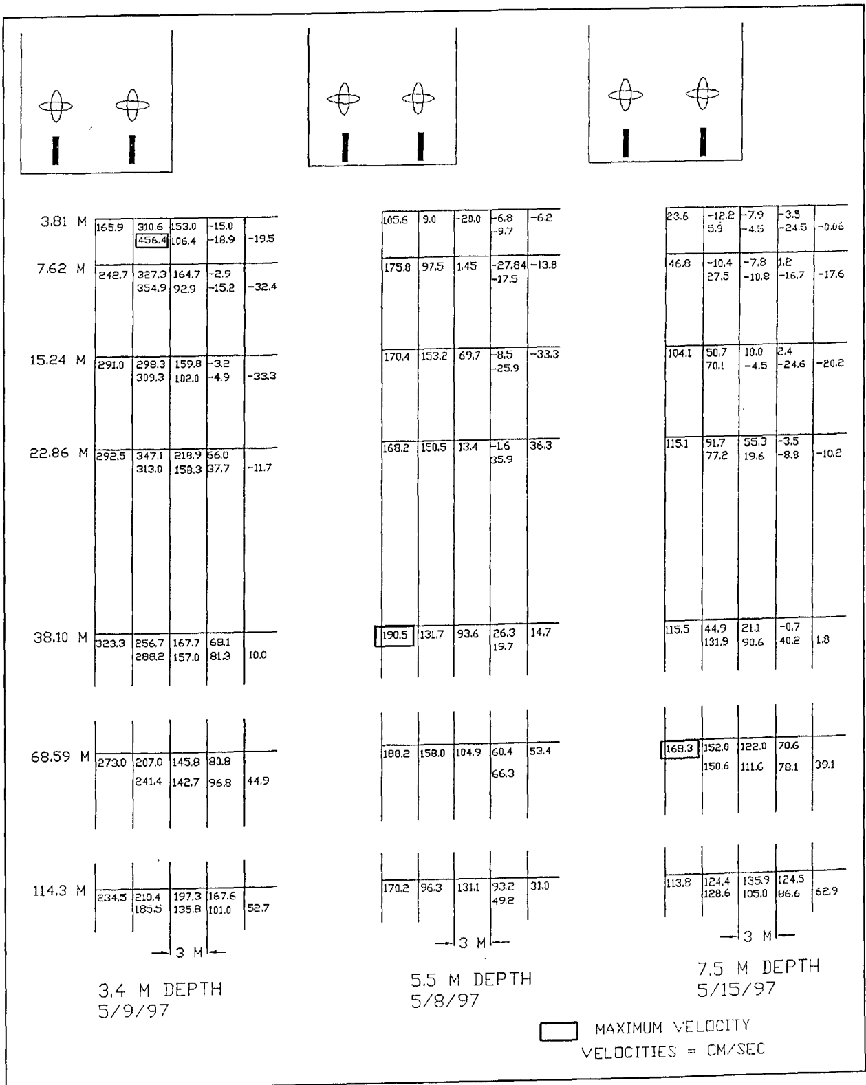
Figure 10. Near-bed propeller jet velocities, open-wheel propellers, stationary tow
