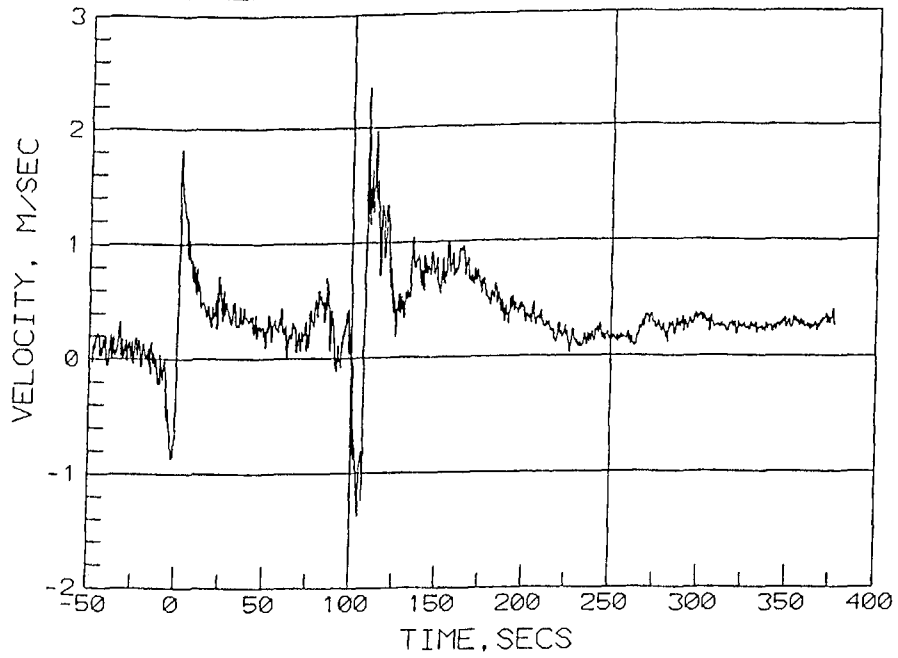
EXPERIMENT KV1524AT VELOCITY TIME HISTORY
