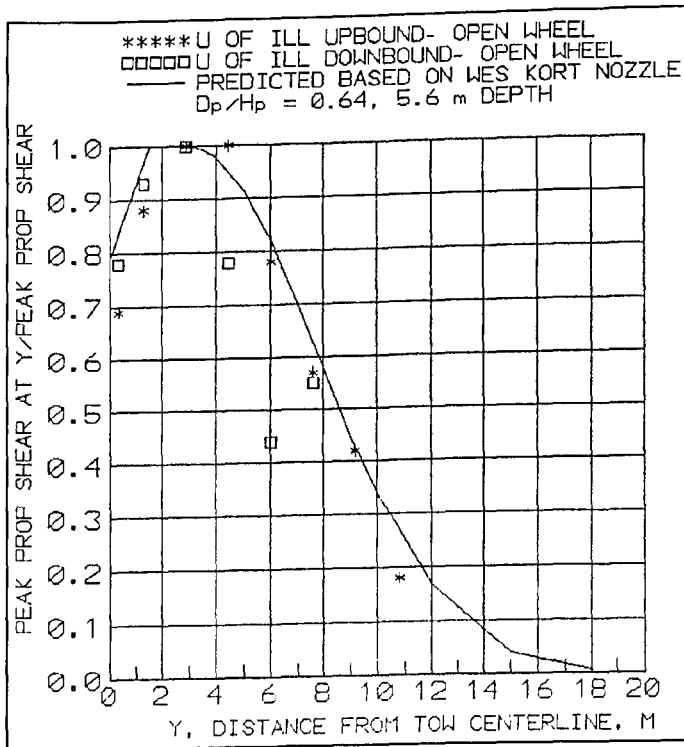
Figure 25. Lateral distribution of peak shear, open-wheel propellers, 5.6-m depth
