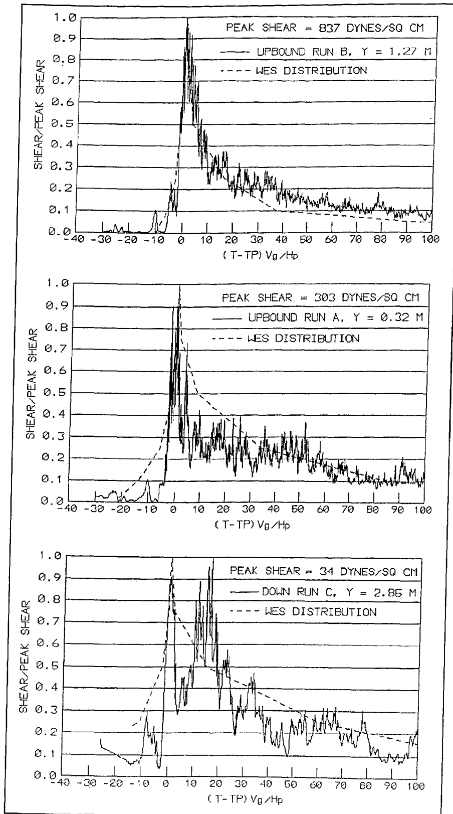
Figure 36. WES Kort nozzle distribution versus Garcia et al. (1998) open-wheel measurements
