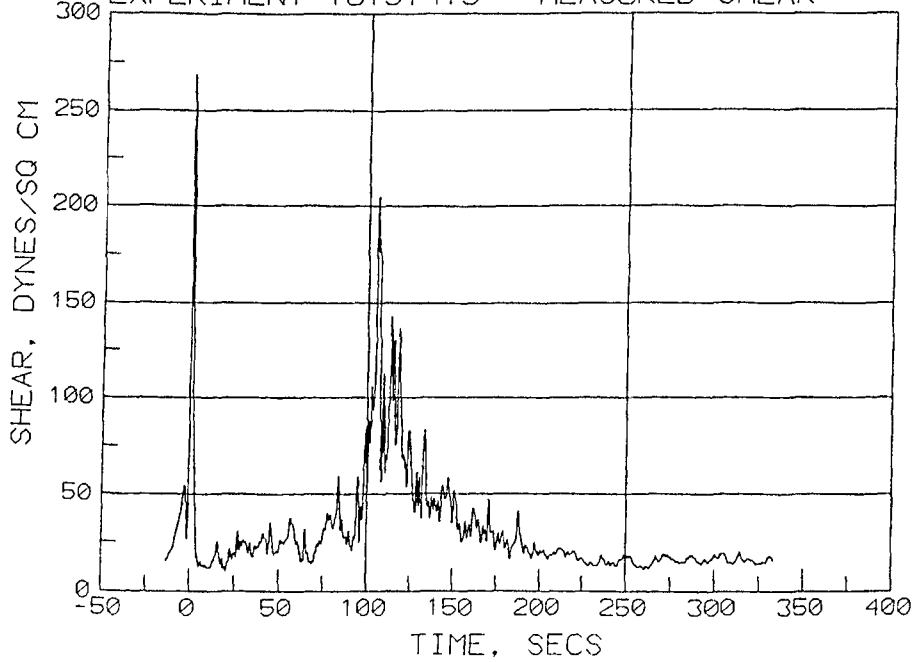
EXPERIMENT TU1514T5 MEASURED SHEAR
