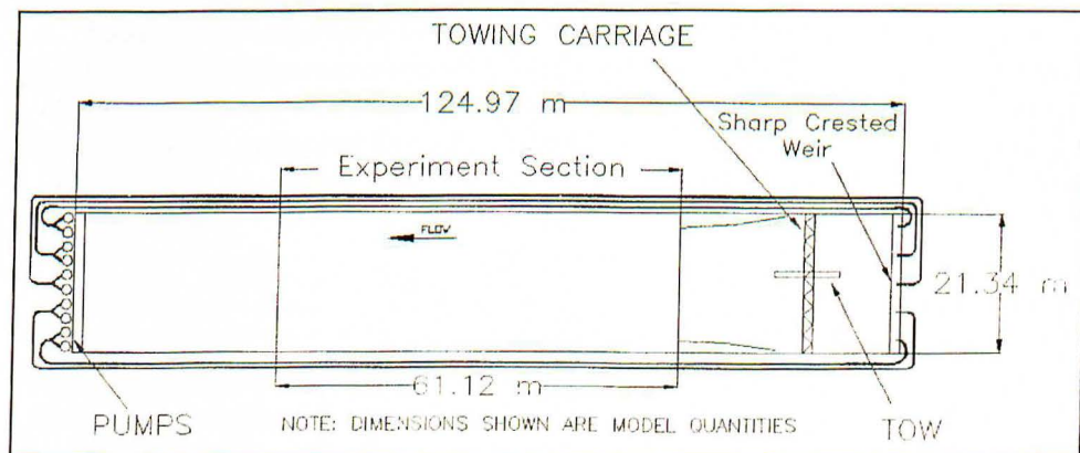
Figure 1. Navigation effects flume
