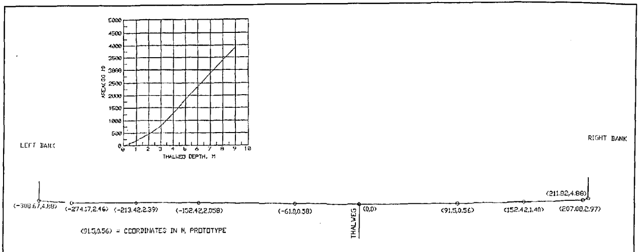
Figure 2. Cross section in experimental section, dimensions expressed as prototype equivalent of 1:25-scale model
