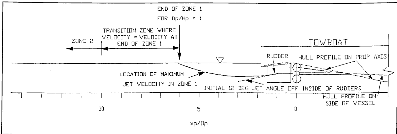
Figure 12. Zone locations for velocity distribution and tunnel stern configuration
