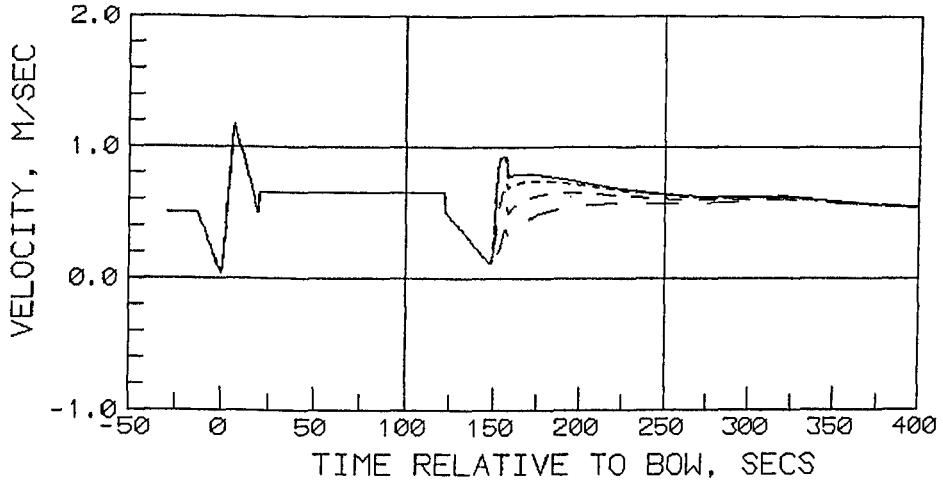
COMPUTED NEAR-BED VELOCITY FOR OPEN WHEEL TOWBOAT INPUT BASED ON EXPERIMENT 0306-2DX
