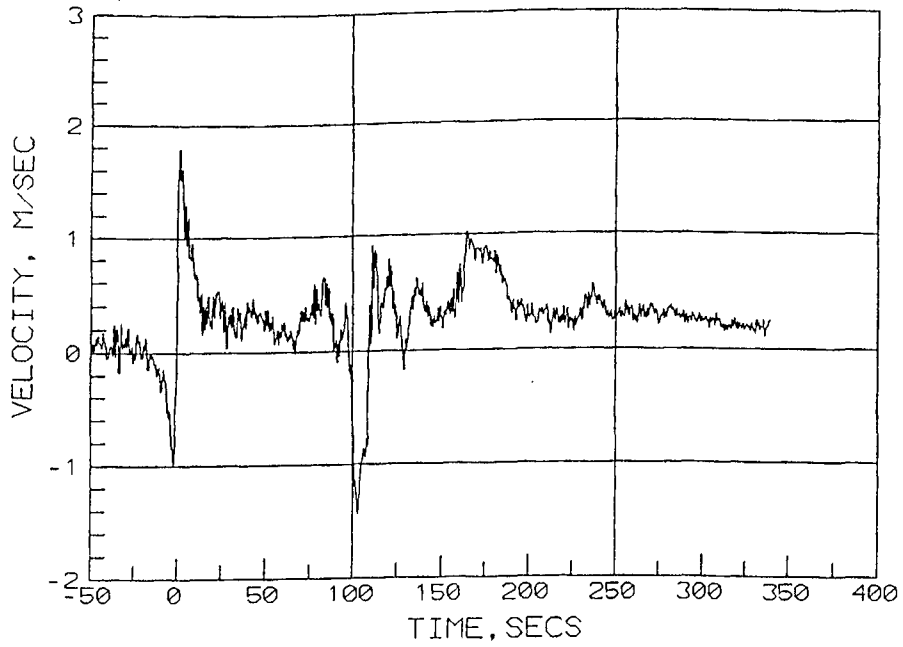
EXPERIMENT KV1534AT VELOCITY TIME HISTORY
