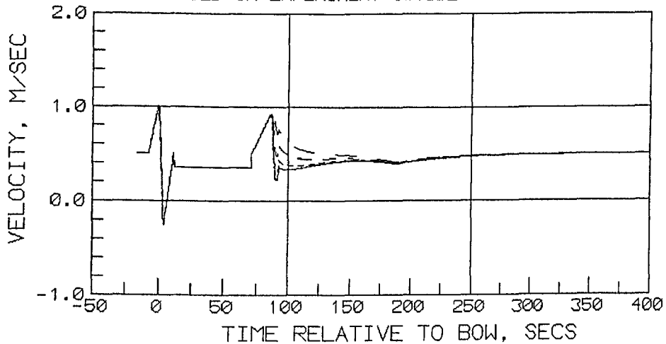
COMPUTED NEAR-BED VELOCITY FOR OPEN WHEEL TOWBOAT INPUT BASED ON EXPERIMENT 0306D2CX
