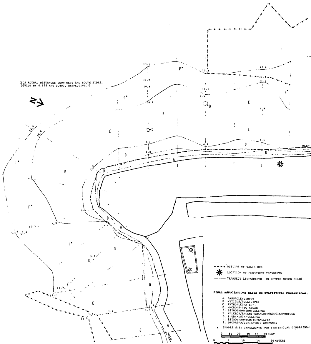
Figure 10. Major species associations, southwest quadrant.
