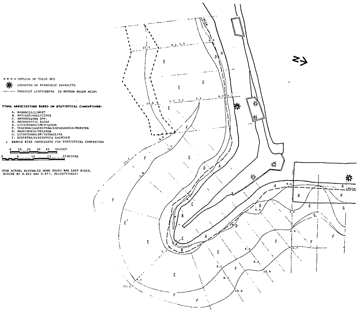
Figure 11. Major species associations, southeast quadrant.
