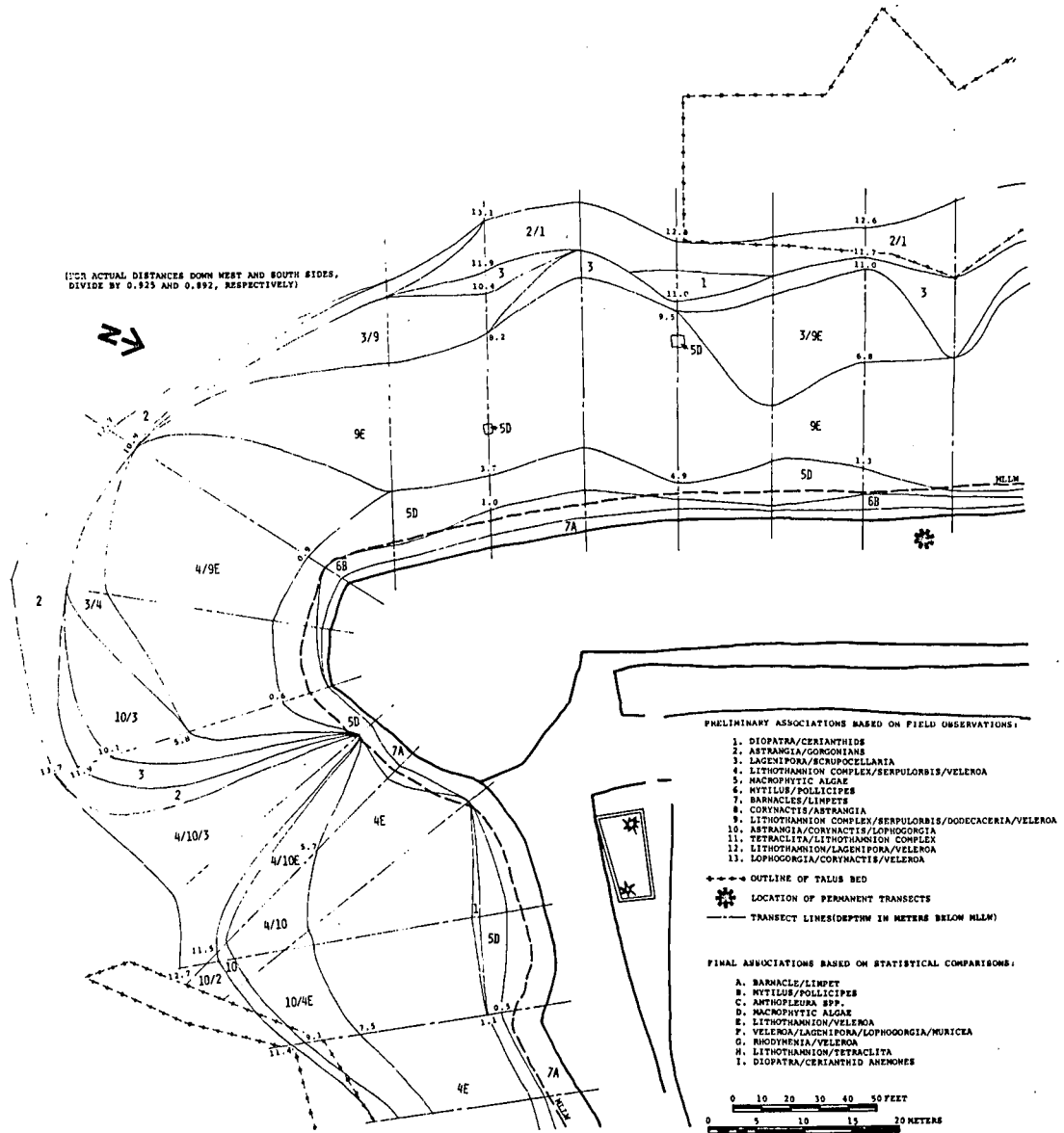
Figure C-4. Preliminary and final special associations, southwest quadrant.
