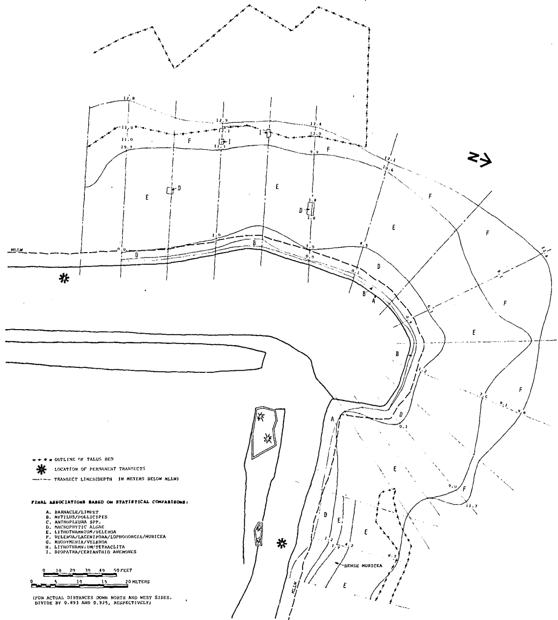
Figure 9. Major species associations, northwest quadrant.
