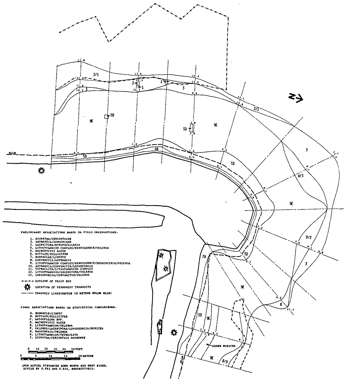
Figure C-3. Preliminary and final species associations, northwest quadrant.
