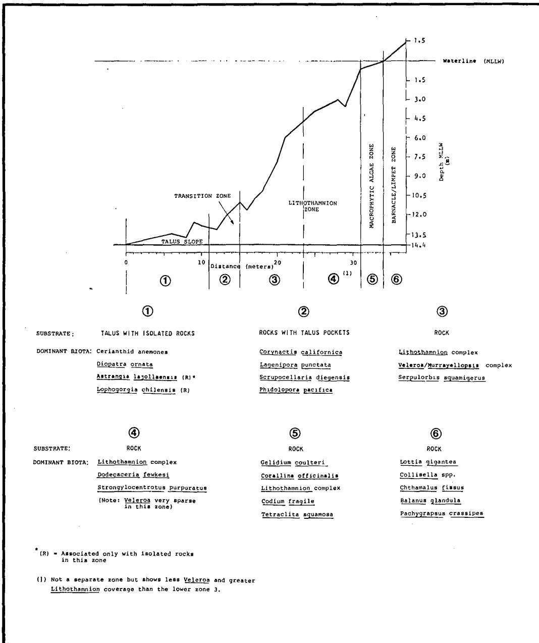
Figure 15. Seasonal overview of distribution of major species associations and substrate character, south-side permanent transect.
