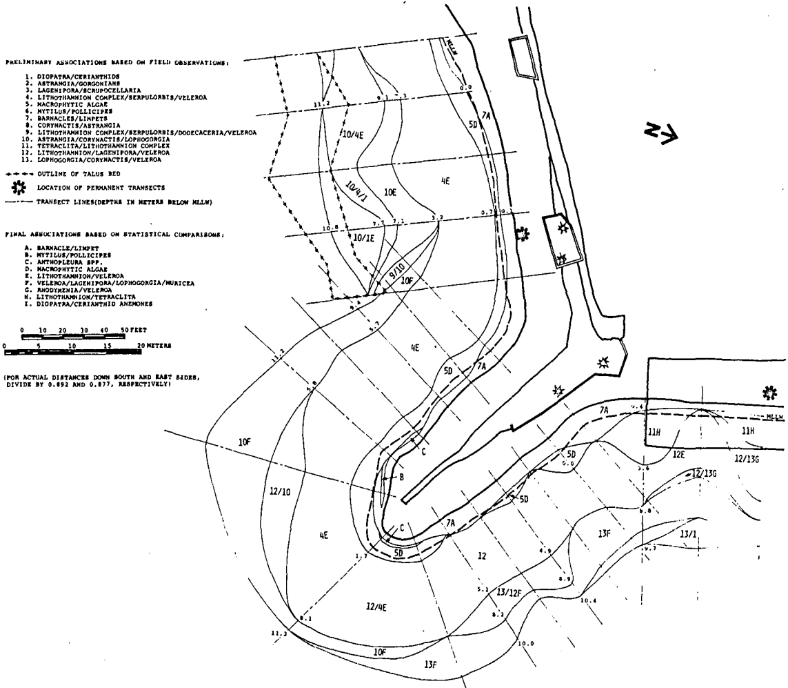
Figure C-5. Preliminary and final special associations, southeast quadrant.
