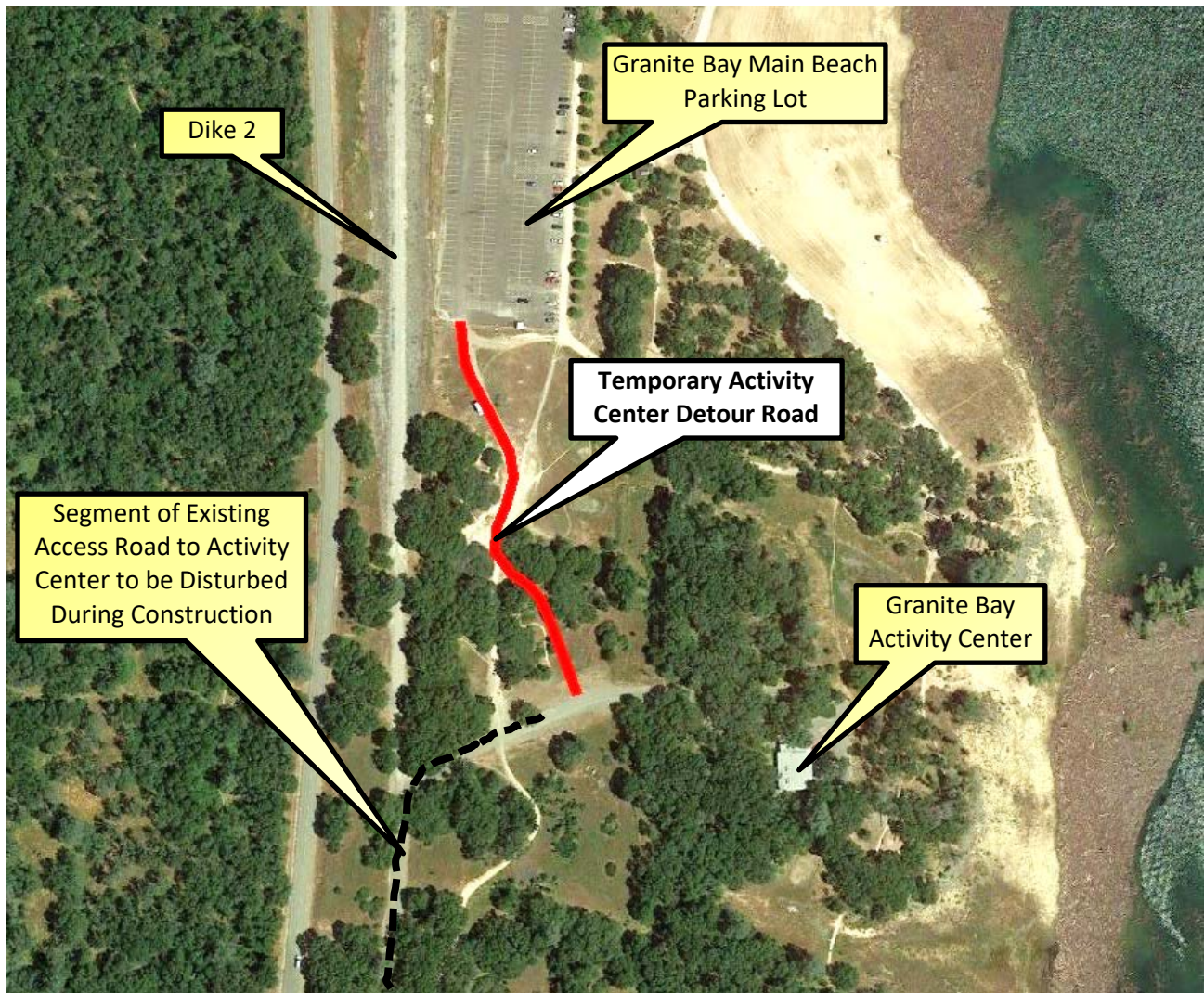
Figure 3-4A. Proposed temporary Granite Bay Activity Center Detour Road alignment.
