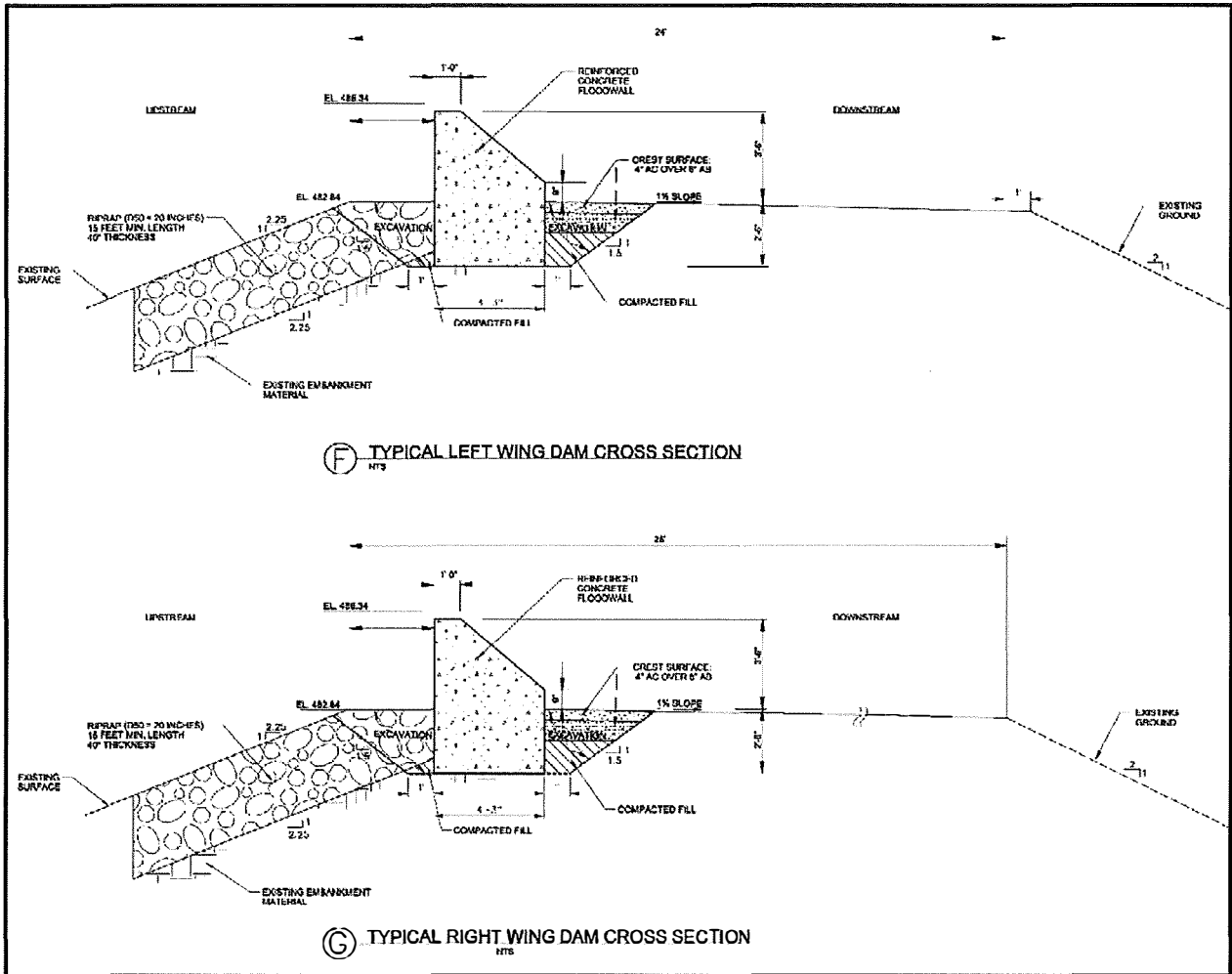
Figure 12. Preliminary typical cross sections for new floodwalls at the Left Wing Dam and the Right Wing Dam.
