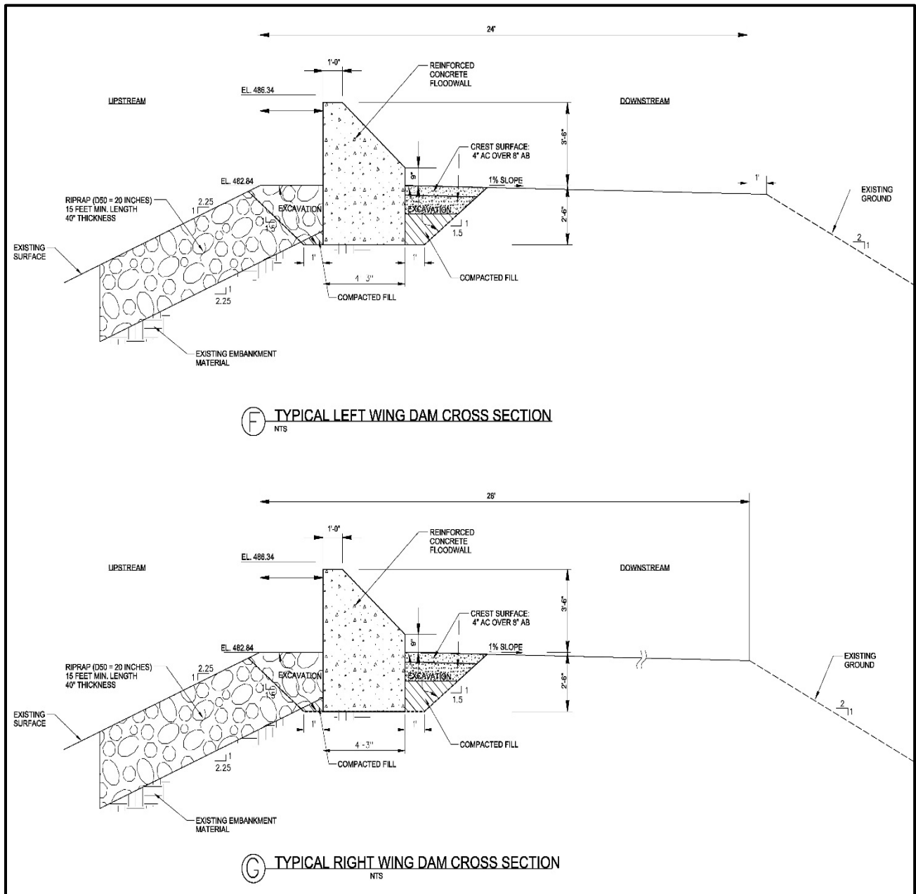
Figure 2-9. Preliminary typical cross sections for new floodwalls at the Left Wing Dam (LWD) and the Right Wing Dam (RWD).
