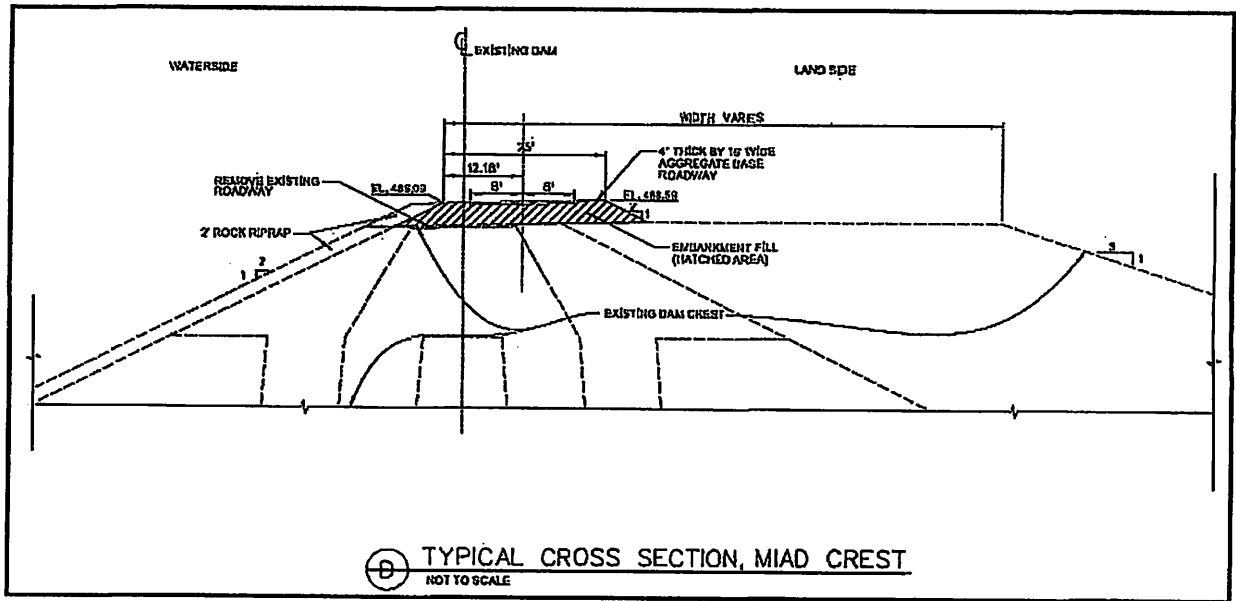
Figure 7. Preliminary typical cross section for 3.5-foot raise at Mormon Island Auxiliary Dam (MIAD).
