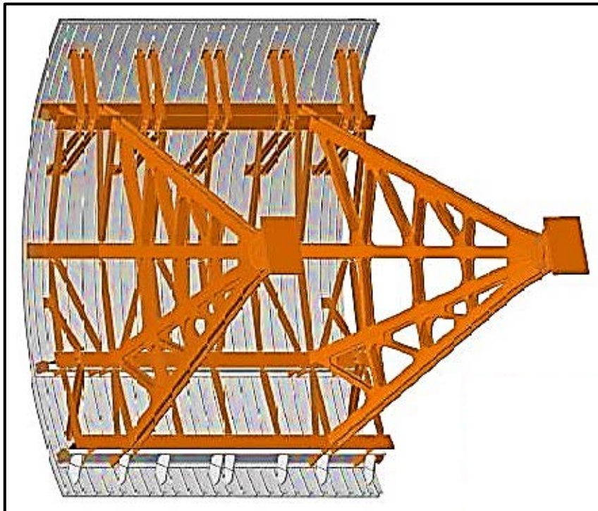
Figure 2-3. Drawing of a typical Tainter gate as viewed obliquely from the downstream side. Curved front panel (shown in gray) faces upstream.
