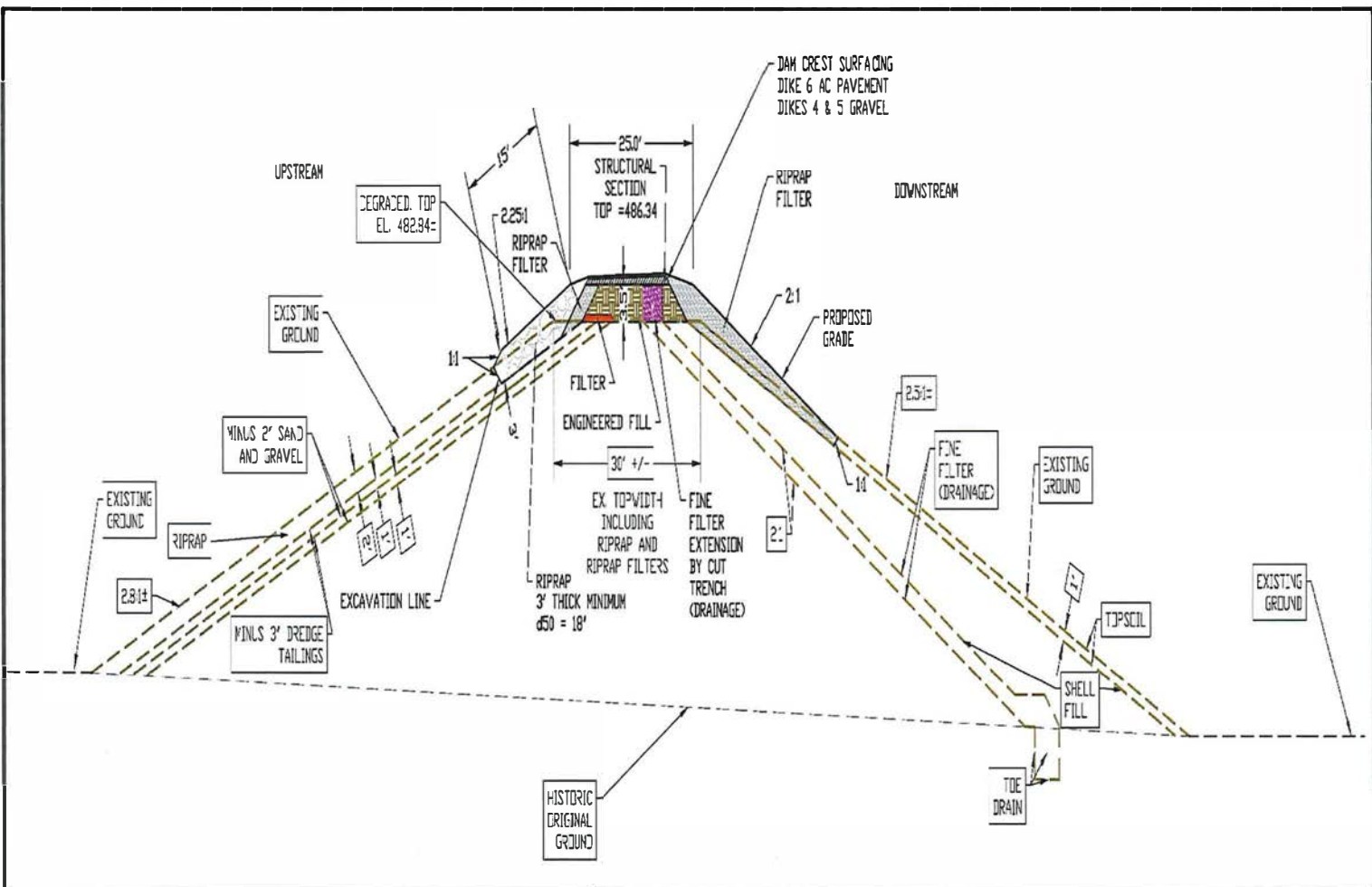
Figure 5. Preliminary typical cross section for 3.5-foot raise at Dikes 4, 5, and 6.
