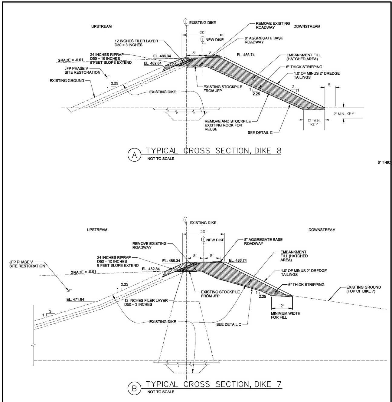
Figure 2-7. Preliminary typical cross section for 3.5-foot raise at Dikes 7 and 8.
