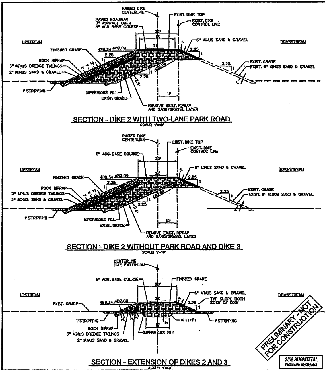
Figure 4. Preliminary typical cross sections for 3.5-foot raise at Dike 2 and Dike 3.
