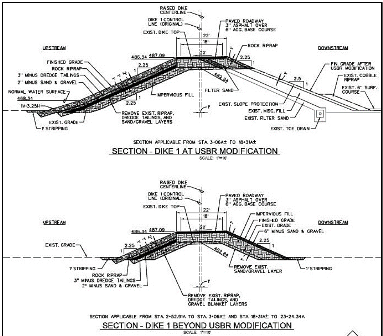
Figure 2-4. Preliminary typical cross section for 3.5-foot raise at Dike 1
