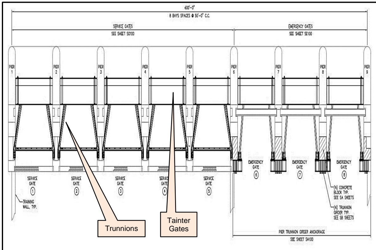
Figure 2-2. Depiction of main dam Tainter gates, trunnions, and associated piers. View from downstream side of dam looking upstream toward dam itself.
