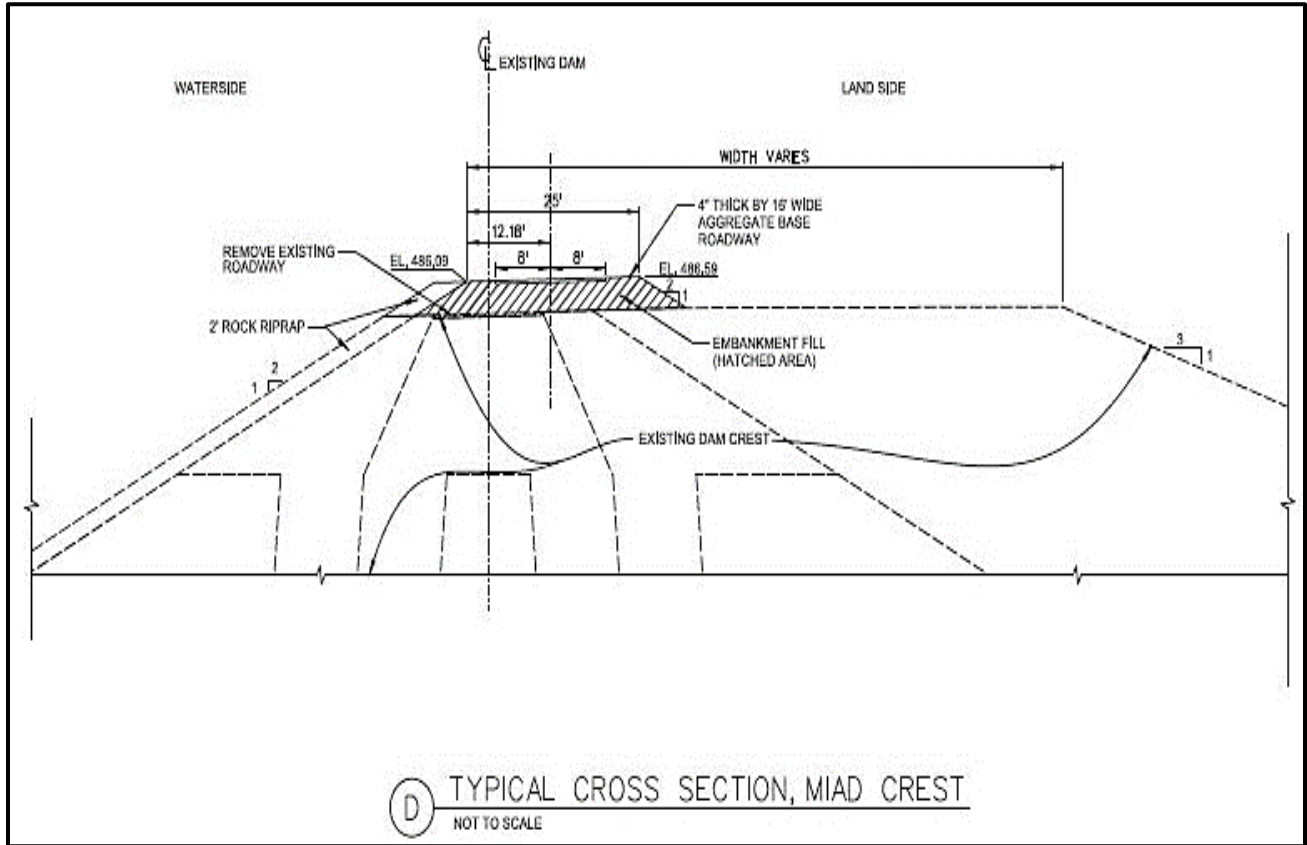
Figure 2-8. Preliminary typical cross section for 3.5-foot raise at Mormon Island Auxiliary Dam (MIAD).
