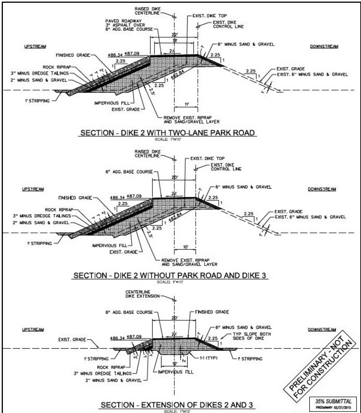
Figure 2-5. Preliminary typical cross section for 3.5-foot raise at Dike 2 and Dike 3.
