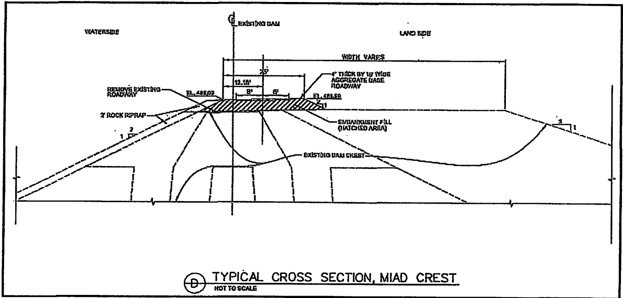
Figure 7. Preliminary typical cross section for 3.5-foot raise at Mormon Island Auxiliary Dam (MIAD).
