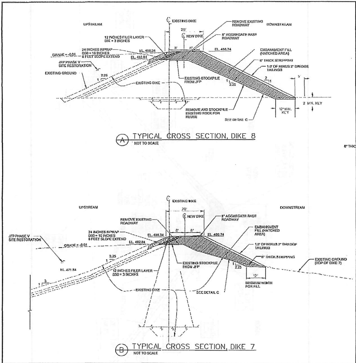
Figure 6. Preliminary typical cross sections for 3.5-foot raise of Dike 7 and Dike 8.
