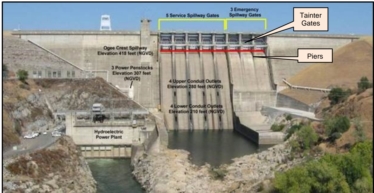
Figure 2-1. Main dam with various existing elements identified.
