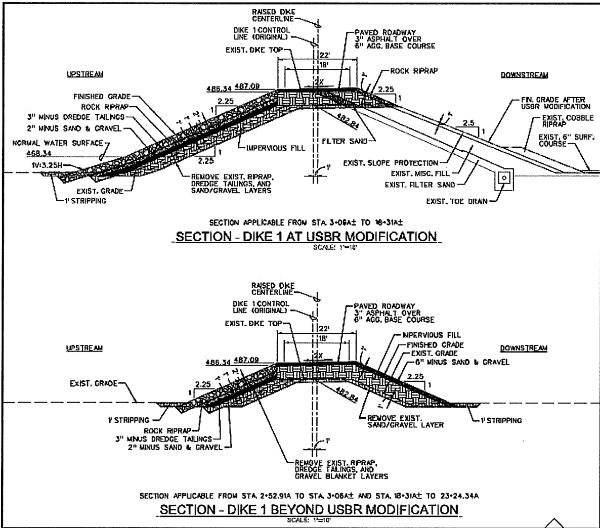
Figure 3. Preliminary typical cross section for 3.5-foot raise at Dike 1.
