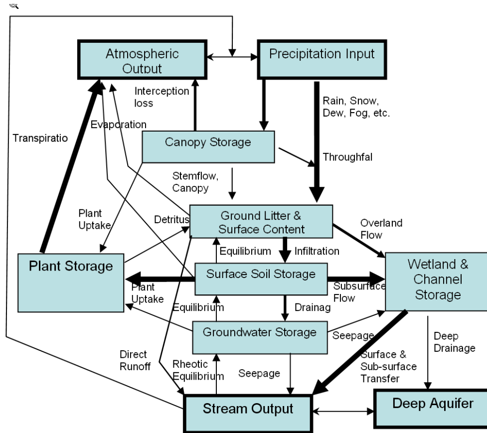
Figure 66. Hydrologic pathway.
