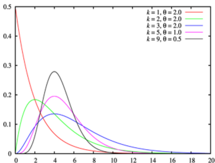
Figure 100. Gamma distributions.
