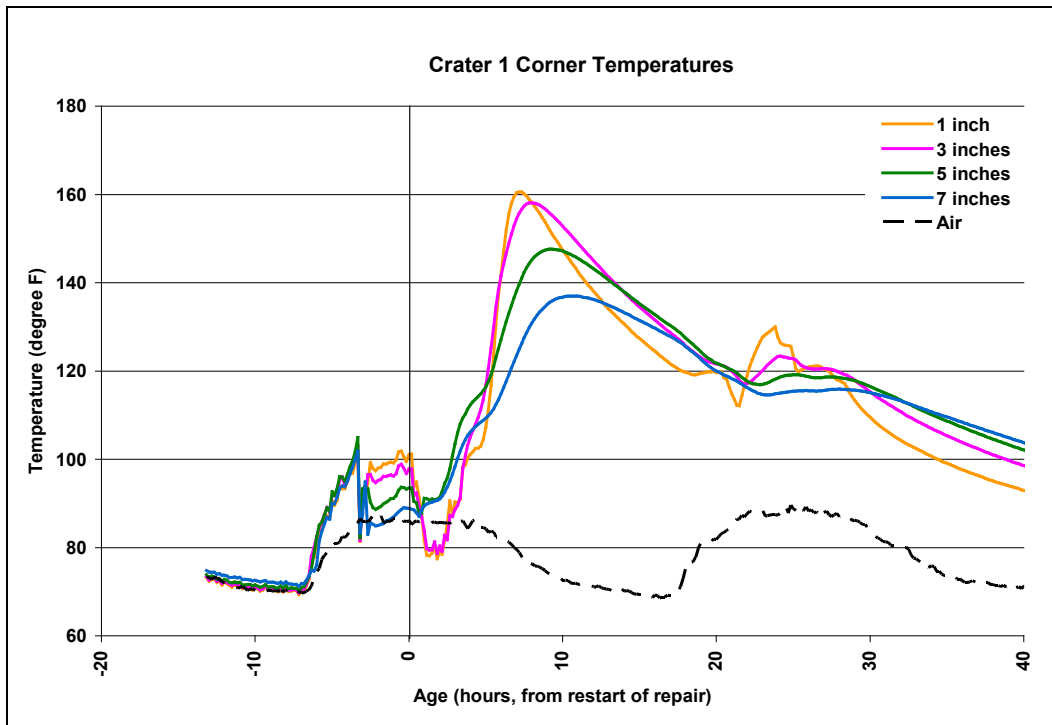
Figure 39. Temperatures in southeastern corner of Crater 1 stone and grout repair.
