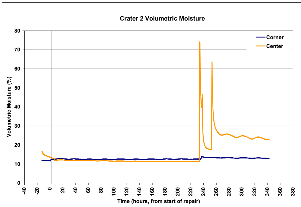
Figure 77. Moisture readings from both center and corner locations in Crater 2.
