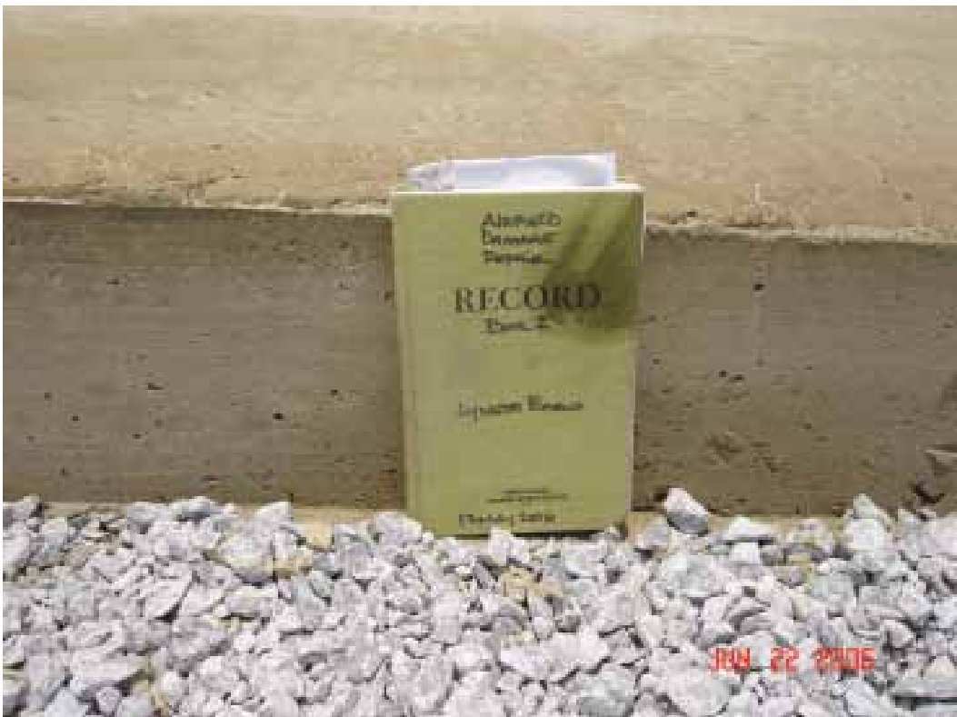
Figure 47. Profile of slab edge of Crater 6 after removal of the form.
