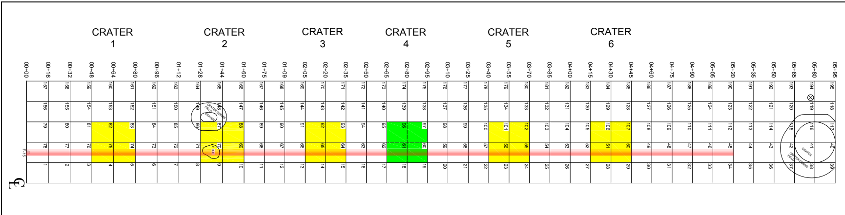
Figure 6. Layout of test area indicating locations of each simulated test crater and load cart trafficking lanes.
