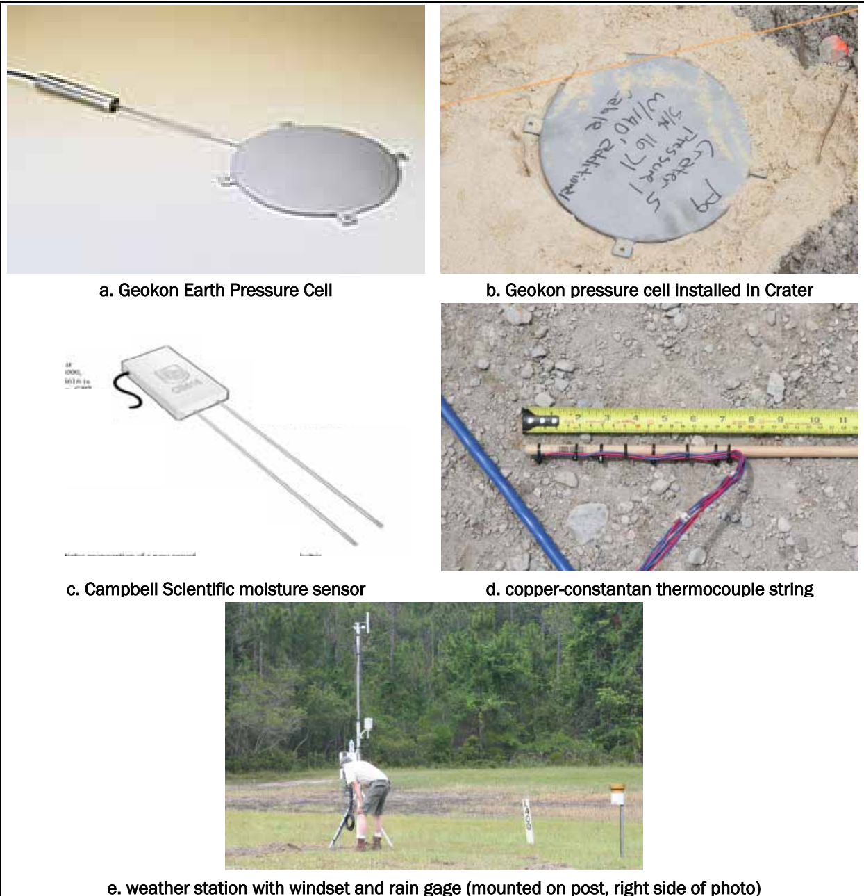
Figure 15. Instrumentation installed in the test craters.
