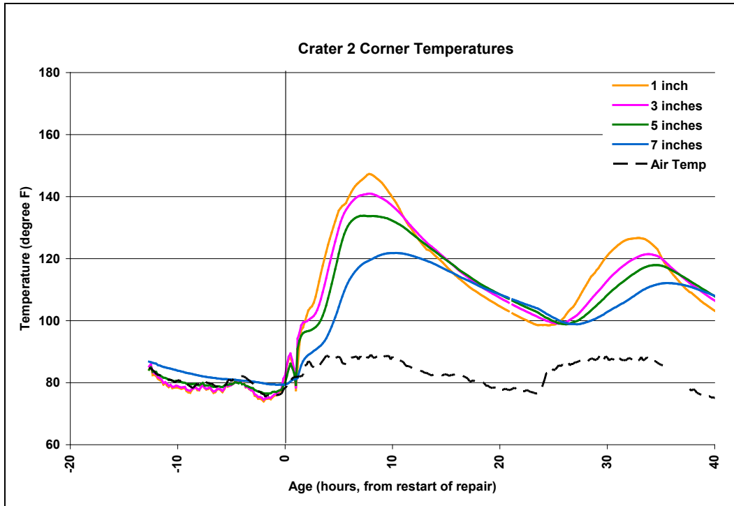
Figure 76. Temperature readings from southeastern corner location of sensors in Crater 2.
