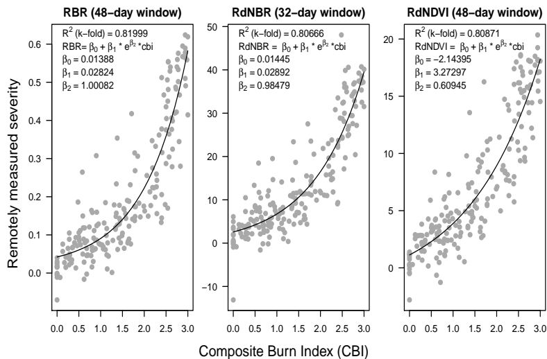
Fig. 4. Three top performing remotely-sensed severity metrics based on 5-fold cross validation (relative burn ratio, 48-day window, bicubic interpolation; relative delta normalized burn ratio, 32-day window, bilinear interpolation; and relative delta normalized difference vegetation index, 48-day window, bilinear interpolation) calculated using new automated image collation algorithms, calibrated to 208 field measures of fire severity (composite burn index). See Supplemental Table 1 for performance of all tested models.
