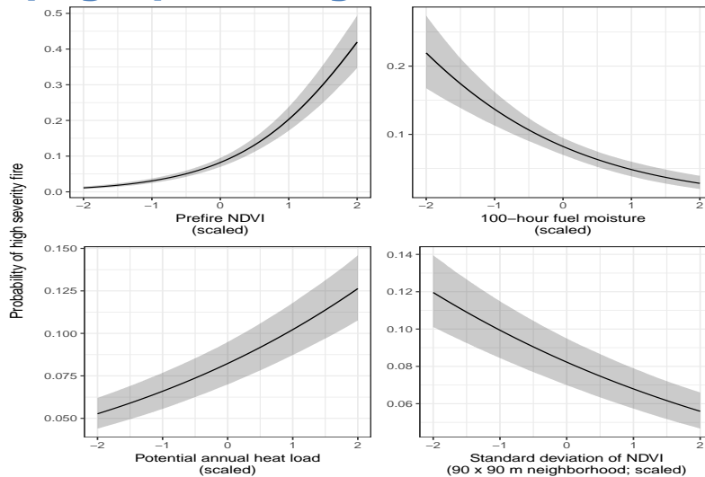
Fig. 5. The main effects and 95% credible intervals of the covariates having the strongest relationships with the probability of high-severity fire. All depicted relationships derive from the model using the 90m x 90m neighborhood size window for neighborhood standard deviation of NDVI, neighborhood mean of NDVI, and topographic roughness, as this was the best performing model of the four neighborhood sizes tested. The effect sizes of these covariates were similar for each neighborhood size tested.
