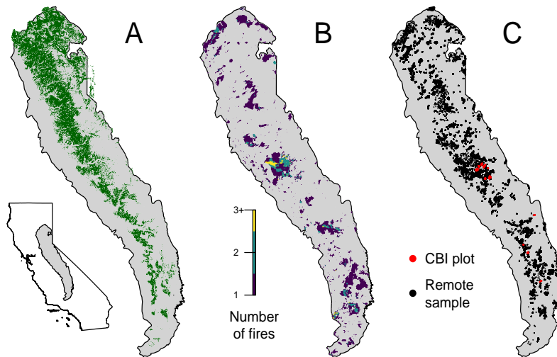
Fig. 1. Geographic setting of the study. A) Location of yellow pine/mixed-conifer forests as designated by the Fire Return Interval Departure (FRID) product which, among other things, describes the potential vegetation in an area based on the pre-Euroamerican settlement fire regime. B) Locations of all fires covering greater than 4 hectares that burned in yellow pine/mixed-conifer forest between 1984 and 2017 in the Sierra Nevada mountain range of California according to the State of California Fire Resource and Assessment Program database, the most comprehensive database of fire perimeters of its kind. Colors indicate how many fire perimeters overlapped a given pixel within the study time period. C) (red) Locations of 208 composite burn index (CBI) ground plots used to calibrate the remotely sensed measures of severity. (black) Locations of random samples drawn from 972 unique fires depicted in panel B that were in yellow pine/mixed-conifer forest as depicted in panel A, and which were designated as “burned” by exceeding a threshold relative burn ratio (RBR) determined by calibrating the algorithm presented in this study with ground-based CBI measurements.
