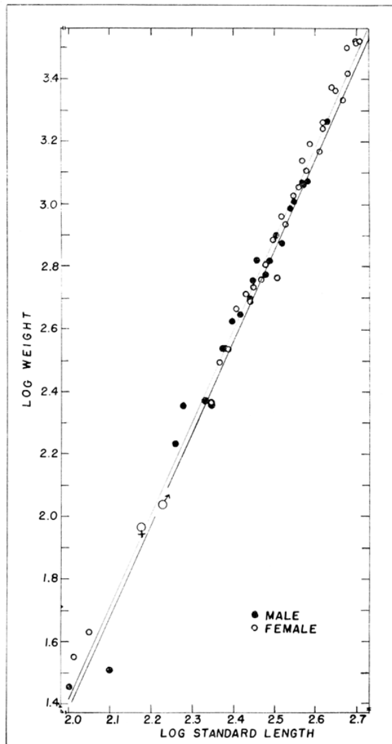
FIGURE 49. Logarithms of weight and length of Platicthys stellatus , Monterey Bay, California
