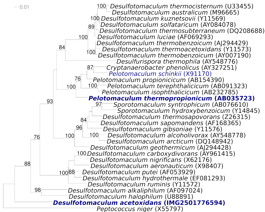
Figure 1. Phylogenetic tree highlighting the position of D. acetoxidans strain 5575 T relative to all type strains of the genus Desulfotomaculum , and the closely related genera Cryptanaerobacter , Desulfurispora , Pelotomaculum and Sporotomaculum , which appear to be nested within the paraphyletic genus Desulfotomaculum . The tree was inferred from 1294 aligned characters [5,6] of the 16S rRNA sequence under the maximum likelihood criterion [7] and rooted with the type strain of the type species of the family Peptococcaceae . The branches are scaled in terms of the expected number of substitutions per site. Numbers above branches are support values from 1000 bootstrap replicates if larger than 60%. Lineages with type strain genome sequencing projects registered in GOLD [8] are shown in blue, published genomes in bold.
