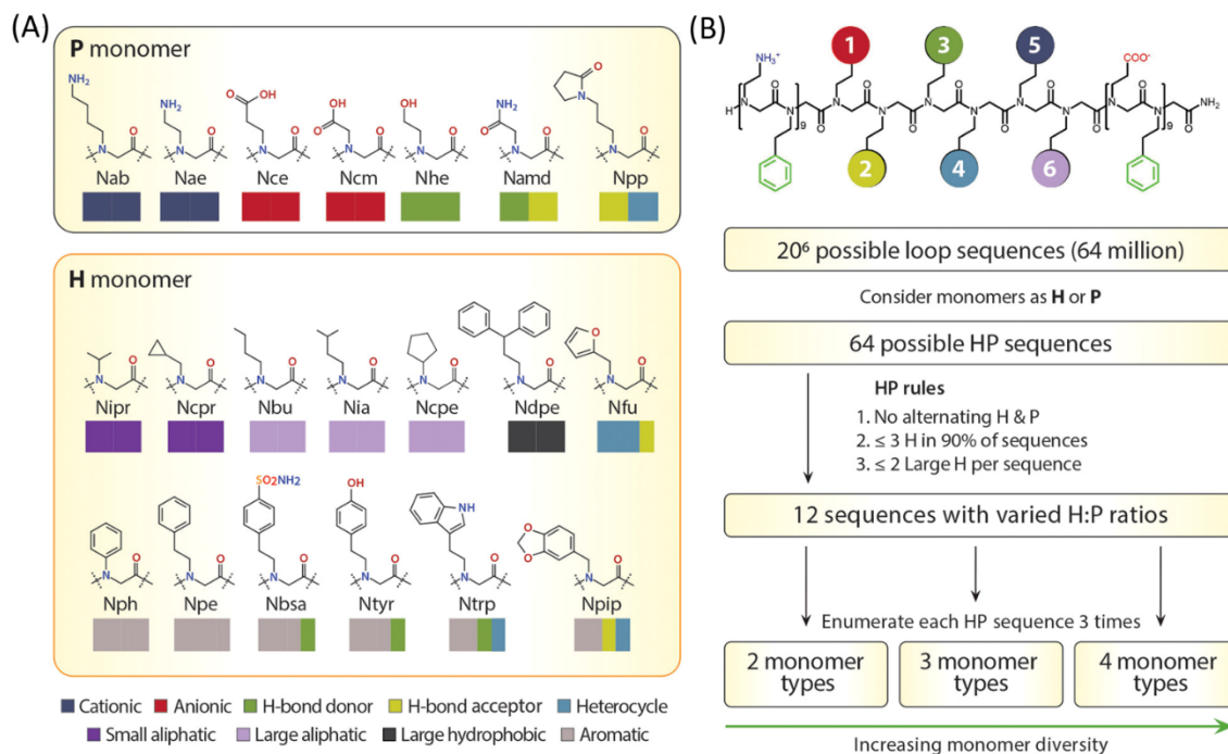
Figure 4. Design of the chemically diverse binding loops, built from a basis of 20 efficiently incorporated monomers. (A) P (hydrophilic) and H (hydrophobic) amine monomers exhibiting various properties. Colored rectangles represent primary and secondary properties of monomers. (B) Design algorithm for creating a maximally diverse set of loop insert sequences, while avoiding extremes of hydrophobicity. Reprinted with permission from Ref. [79]. Copyright (2020) American Chemistry Society.
