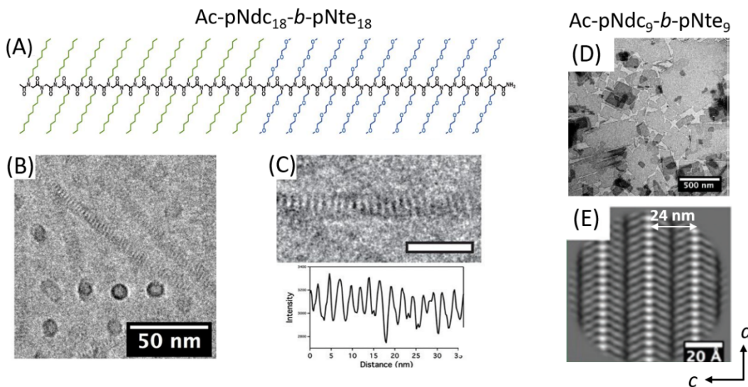
Figure 5. (A) Chemical structure of Ac-pNdc 18 -b-pNte 18 . (B) Cryo-EM 2D projection image shows nanotubes of uniform diameter in a vitrified thin film. (C) Cryo-EM close-up of a single nanotube (scale bar, 20 nm) shows regular latitudinal stripes (Top). A line profile along the longitudinal direction of the nanotube indicates a periodicity of 2.4 \pm 0.2 nm (Bottom). (D) TEM images of nanosheets formed by Ac-pNdc 9 -b-pNte 9 . (E) Cryo-TEM image of the nanosheets showing a 24 nm spacing between adjacent rows of backbones along the c direction. (D) is adapted with permission from Ref. [51]. Copyright (2018) American Chemistry Society. (E) is adapted from Ref. [52]. with permission from The Royal Society of Chemistry.
