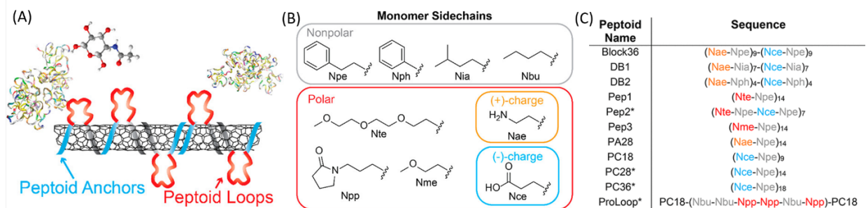
Figure 6. Electrostatic assemblies of single-walled carbon nanotubes (SWNT) and peptoids. (A) A cartoon showing adsorption of peptoids onto the surface of SWNT with peptoid loops well displaced for the detection of a lectin protein. (B) Monomers used to create the peptoids in this study. (C) Library of 11 Peptoid structures tested for adsorption to SWNT. Peptoids denoted with an asterisk (*) successfully adsorb on SWNT to form peptoid-SWNT assemblies, while other peptoids do not suspend SWNT at pH 7. Adapted with permission from Ref. [81]. Copyright (2019) American Chemistry Society.
