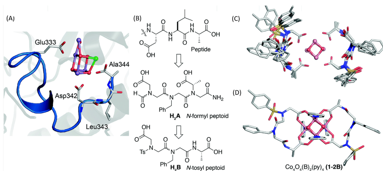
Figure 8. (A) Selected amino acid residues from the D1 subunit (blue) that bind to the Mn 4 Ca oxygen-evolving complex (OEC). (B) Design of the peptoid analogues based on D1. (C) Ensemble of the five lowest energy NMR structures of 1-2B (pyridine ligands omitted for clarity). (D) The lowest energy structure of 1-2B . Reprinted from Ref. [91]. with permission from The Royal Society of Chemistry.
