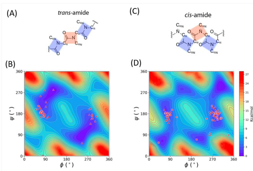
Figure 2. Ramachandran plots of peptoids representing \phi and \psi from 0^\circ to 360^\circ . (A) Line drawing of trans -amide backbone conformations in peptoids. (B) Free-energy plot of trans disarcosine and \phi and \psi combinations derived from trans -amide conformations in peptoid X-ray crystal structures ( \blacktriangle ) and NMR structures (X). (C) Line drawing of cis -amide backbone conformations in peptoids. (D), Free-energy plot of cis disarcosine and \phi and \psi combinations derived from cis -amide conformations in peptoid X-ray crystal structures ( \blacktriangle ) and NMR structures (X). Adapted with permission from Ref. [61] Copyright (2019) John Wiley and Sons.
