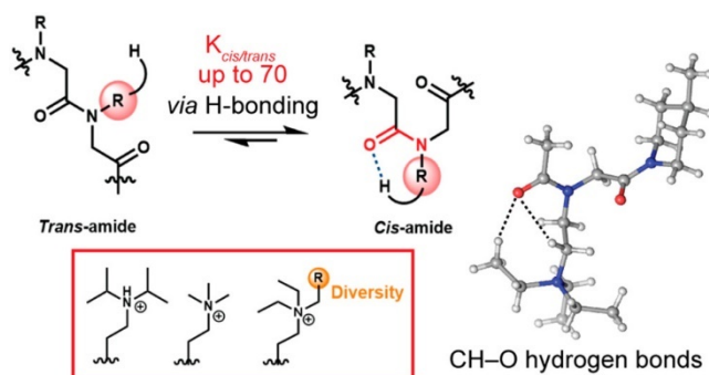
Figure 9. Cationic alkyl ammonium ethyl side chains, highly diverse, induced cis -amide conformation of peptoids through an ensemble of weak CH-O hydrogen bonding. The K_{cis/trans} could reach up to 70. Reprinted with permission from Ref. [97]. Copyright (2019) American Chemistry Society.
