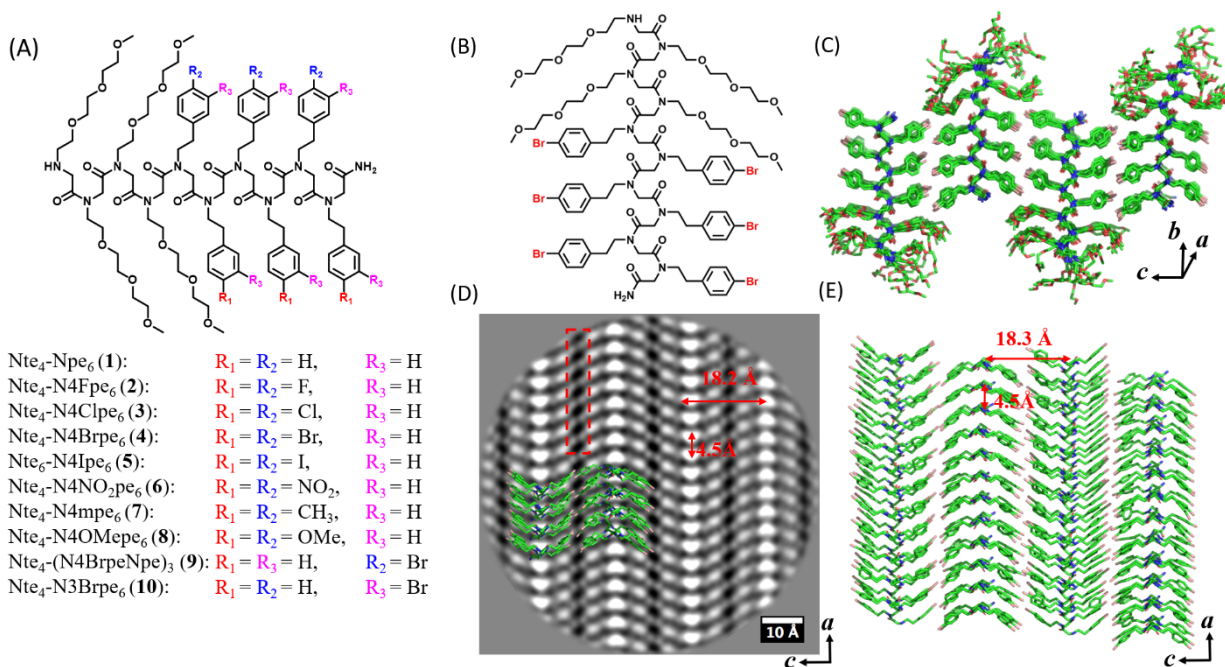
Figure 3. Atomic engineering of nanosheets. (A) Chemical structures of diblock copolypeptoids with various para -substituents of aromatic side chains. (B) Chemical structures of Nte 4 -N4Brpe 6 (4). (C) Molecular model of sheet 4. The molecules are packed antiparallel along c direction and parallel along a direction. (D) Cryo-TEM image of sheet 4 from b direction (top view) showing anti-parallel V shapes along the c direction. The Br atoms showed a tip-to-tip packing (red box). (E) Top view of the hydrophobic domain in (C) from b direction showing anti-parallel V shapes along the c direction. The structure is overlapped with cryo-TEM image shown in (D).
