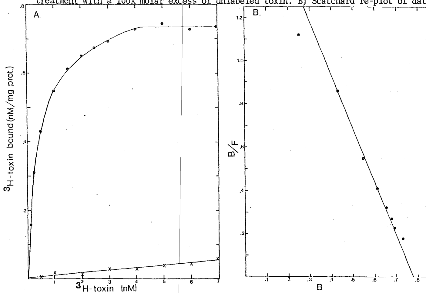
Figure 5-5 Saturation of ^3\text{H} - \alpha -bgt binding to Torpedo nAChR-rich membranes. A) linear plot of specific (---) and non-specific binding (-X-X-) as a function of ^3\text{H} -toxin concentration. Specific binding was given by (total minus non-specific) where the total binding was measured after 60 min incubation at 21°C, followed by a 30 min chase with a 100X molar excess of unlabeled toxin, and the non-specific binding was defined by a 30 min pre-treatment with a 100X molar excess of unlabeled toxin. B) Scatchard re-plot of data in A).
