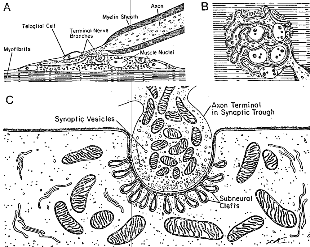
XBL 764-1125 Figure 1-3. Mammalian skeletal neuromuscular junction. A: Side view of a single junction at low magnification. B: Surface view of terminal branching of a motorneuron onto a muscle. C: EM view.
