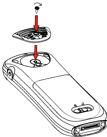
Figure 12. Screw the cover into position.
