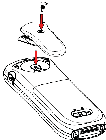
Figure 10. Screw the hinge-type clip into position.
