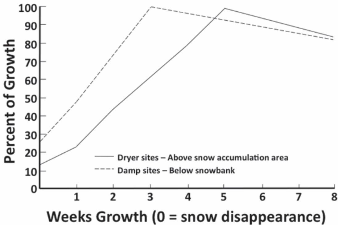
Figure 7.9. Growth curves of alpine plants (from Lewis, 1970).
