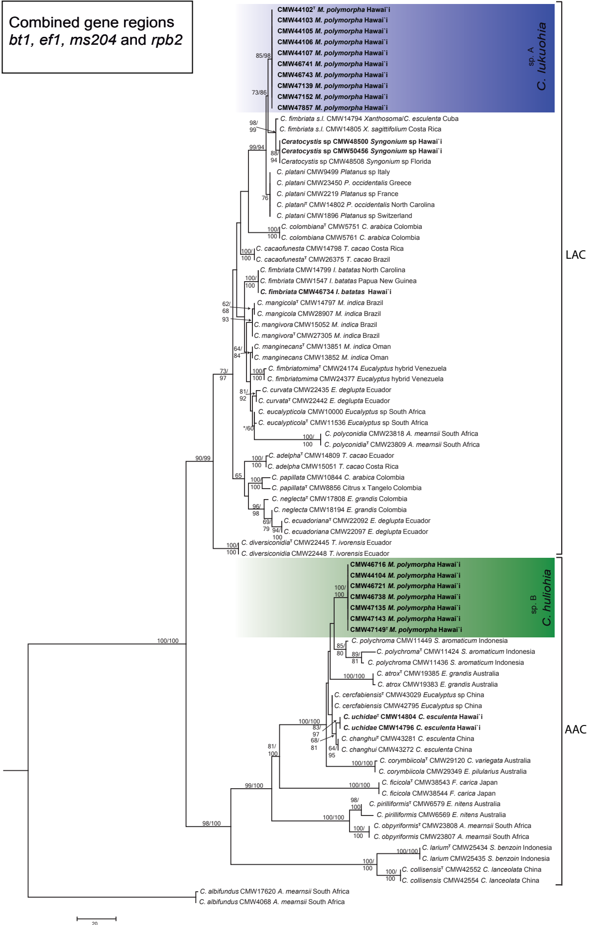
Fig. 4 Maximum parsimony tree based on the combined dataset of four gene regions ( bt1, tef1, ms204 and rpb2 ) for species in the Latin American clade (LAC) and the Asian-Australian clade (AAC) of Ceratocystis . Isolates sequenced in this study from M. polymorpha in Hawaii are highlighted in blue in the LAC, as C. lukuohia (sp. A), and in green in the AAC, as C. huliohia (sp. B). Bootstrap values > 60 % for MP/ML are presented at the branches. Bootstrap values lower than 70 % are indicated with *. Ceratocystis albifundus (CMW 4068) from the African clade was used as the outgroup.
