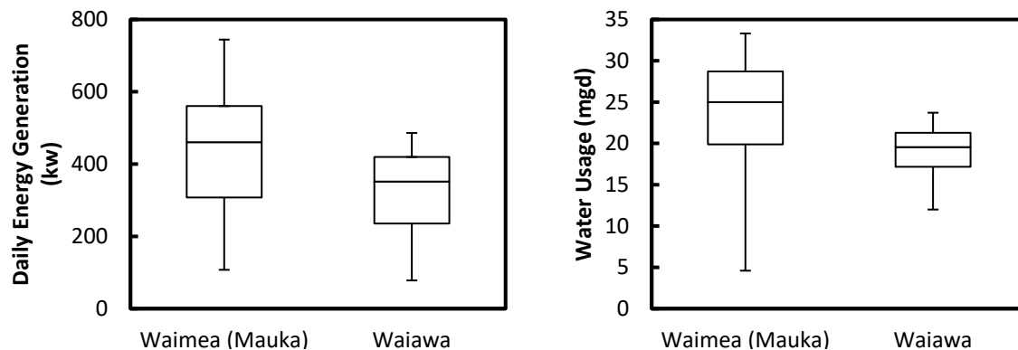
Figure 13-7. Box-and-whisker plots of daily energy generation (left) and daily water usage (right) the Waimea (Mauka) and Waiawa hydropower plants on the Kekaha Ditch. (Source: Kekaha Agriculture Association, 2015)
