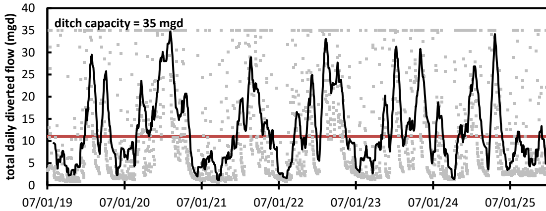
Figure 13-14. Mean daily simulated diverted flow into Kokee Ditch after contributions from Waiakoali Stream, Kawaikoi Stream, and Kauaikinana Stream (grey dots), 30-day moving average (black line), and the 11 mgd reference (red line) from 07/01/1919 to 12/31/1925.
