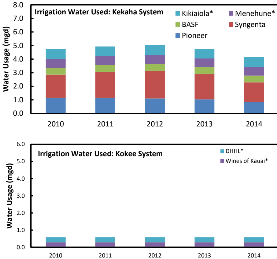
Figure 13-11. Mean daily irrigation water usage for primary users of the Kekaha (top) and Kokee (bottom) irrigation systems from 2010 to 2014 (Source: Kekaha Agriculture Association, 2015). *values estimated
