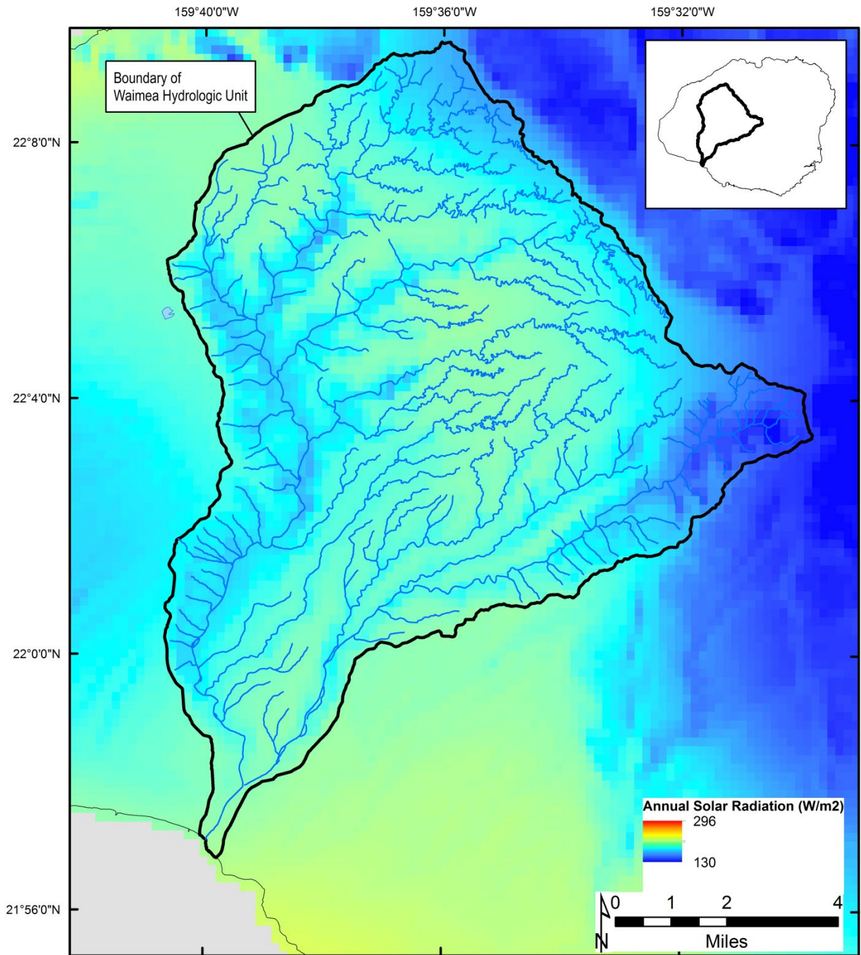
Figure 2-5. Mean annual solar radiation for the Waimea hydrologic unit. (Source: State of Hawaii, Office of Planning, 2015c)
