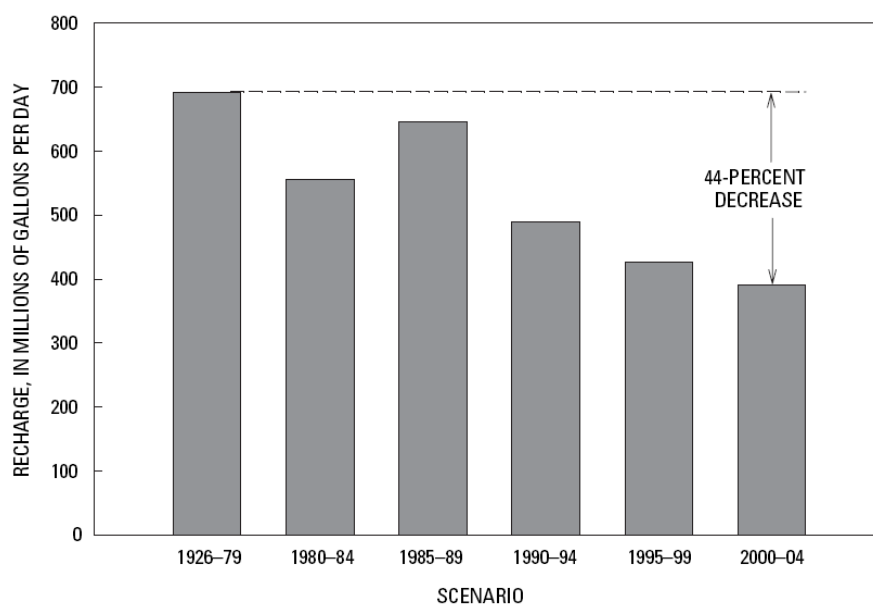
Figure 13-2. Estimated recharge for six historical periods between 1926 and 2004, central and west Maui, Hawaii. (Source: Engott and Vana, 2007)
