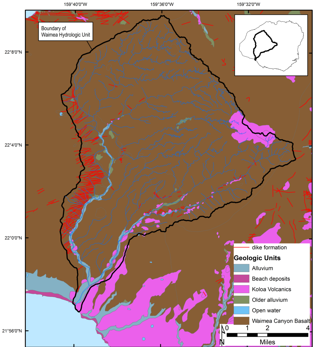
Figure 2-1. Generalized geology of Waimea hydrologic unit. (Source: Sherrod et al., 2007)
