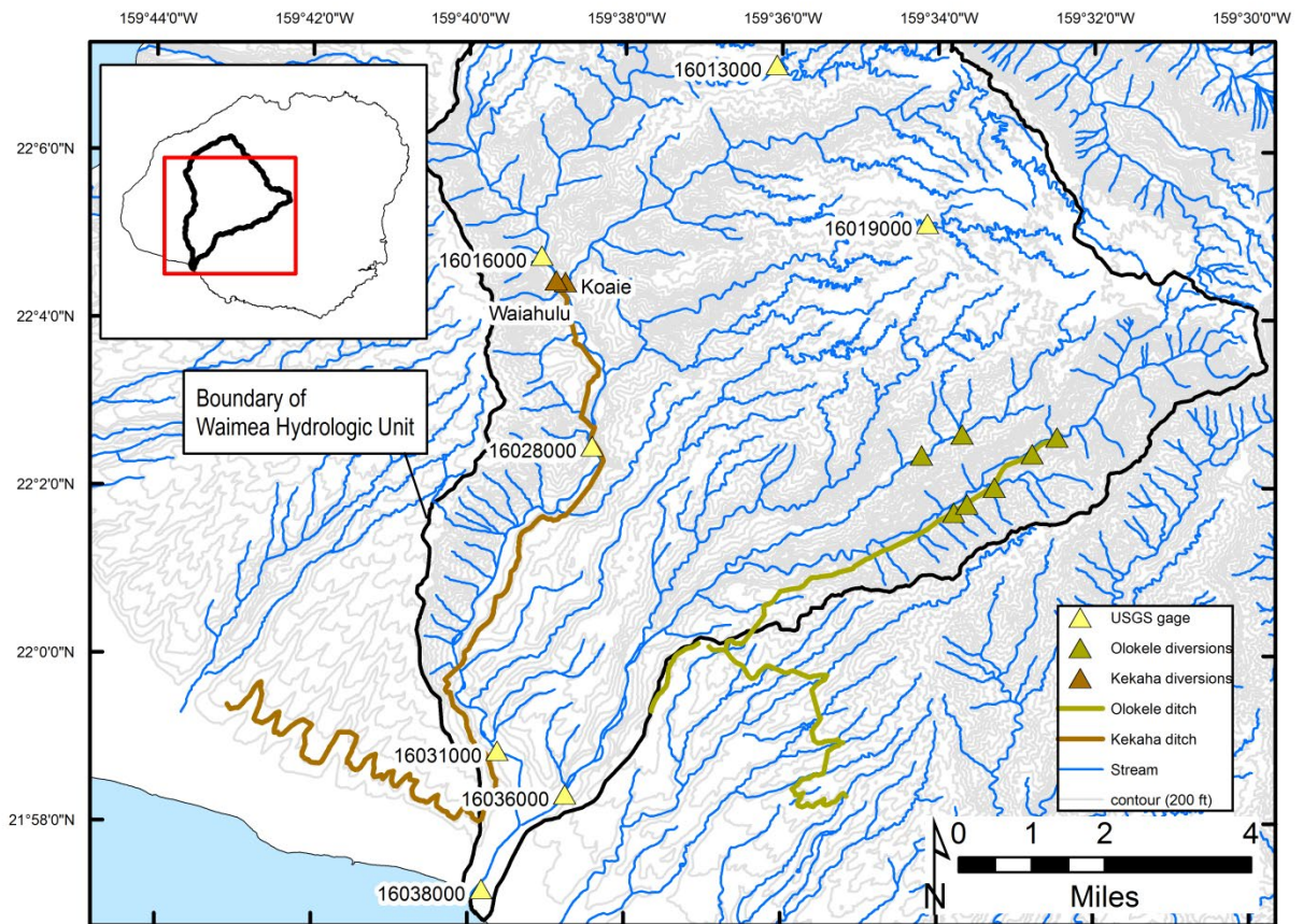
Figure 3-3. Ditches, diversions and gaging stations in the lower Waimea hydrologic unit that feed the Kekaha and Olokele ditch systems. (Source: State of Hawaii, Office of Planning, 2004c; State of Hawaii, Commission on Water Resource Management, 2015a; 2015e)
