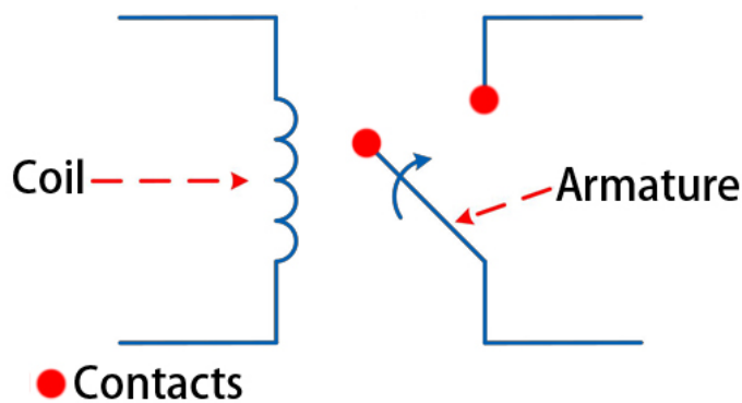
Figure 6. Electromechanical Relay
