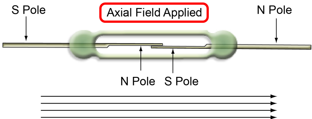
Figure 8. Reed Relay
