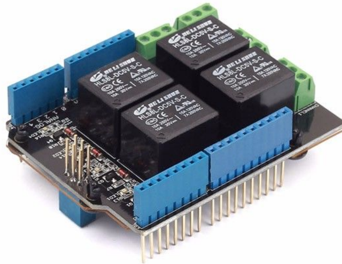
Figure 9. Relay Shield, you can click this figure to check
