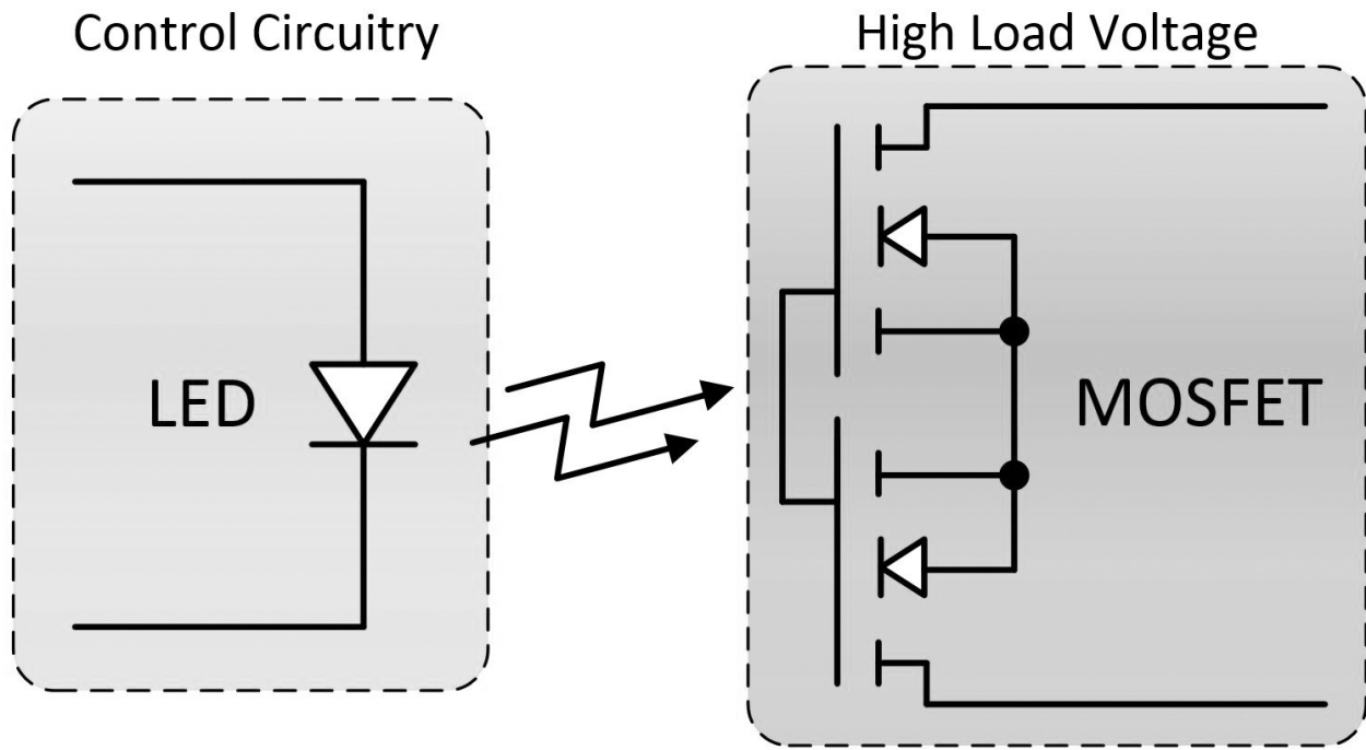
Figure 7. Solid State Relay
