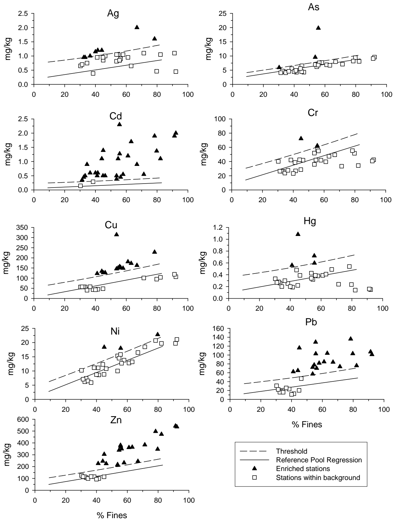
Figure B2. %Fines:metals plots from Chollas and Paleta Creek stations overlaid on the threshold and regression lines from the Baseline Pool. Sites which fall below the threshold are considered uncontaminated. Sites which lie above the threshold are considered enriched.
