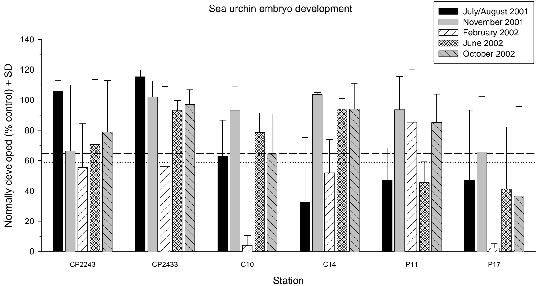
Figure 15. Sea urchin embryo development in quarterly sediment-water interface samples. Data are control adjusted. The dashed line is the lower 95% prediction limit from the Baseline Pool. The dotted line is the 59% normal development threshold.
