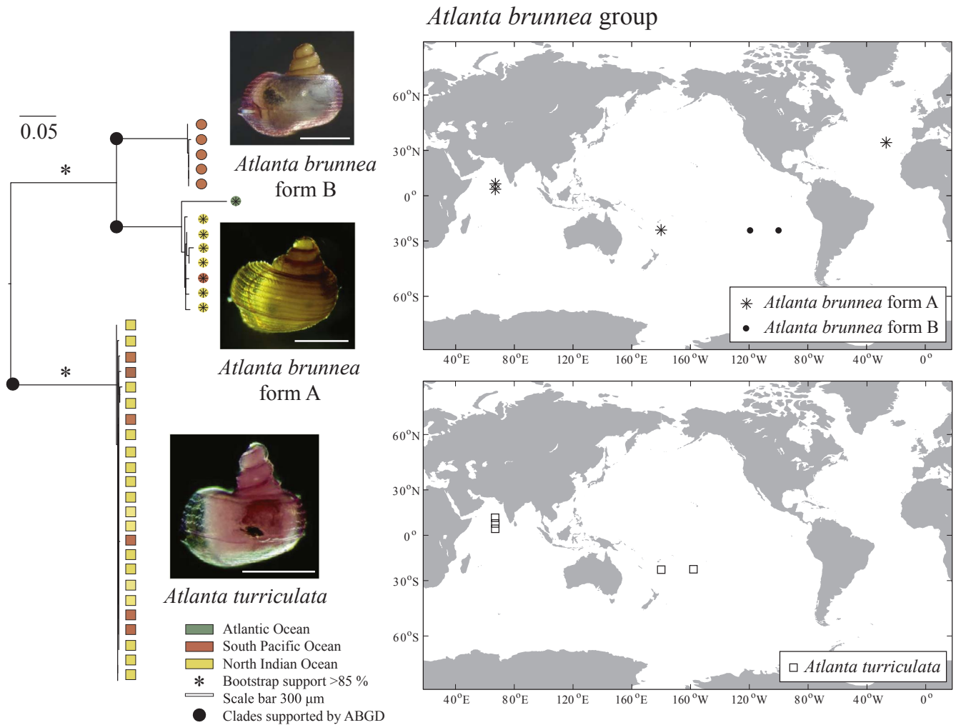
Fig. 3. Maximum likelihood tree showing relationships within the A. brunnea species group. Branches with bootstrap support > 85% are denoted with a star. Branch lengths are proportional to the amount of inferred change, as indicated by the scale bar. Black circles at nodes represent clades supported by ABGD analysis. Maps show the biogeographic position of sequenced specimens with different symbols for each clade. Images demonstrate the morphology of representative sequenced specimens. See Plates 1 and 2 for detailed morphological differences of morphospecies.
