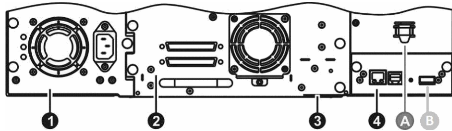
Figure 1-4: NEOs T24 Tape Library (2U) Rear Panel
