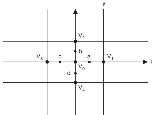
Fig. 0.1 A portion of a region containing a two-dimensional potential field divided into square of side h .
