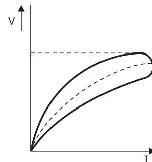
Fig. 7.41 Volt-ampere characteristic of valve-type LA
