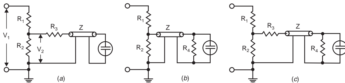
Fig. 4.19 Various forms of resistance potential dividers recording circuits (a) Matching at divider end (b) Matching at Oscillograph end (c) Matching at both ends of delay cable
