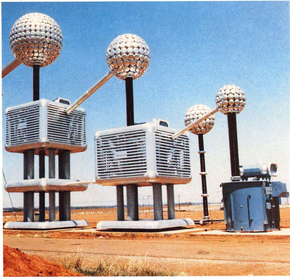
Three-stage cascade transformer 3 x 600 kV, 2 A cont. outdoor type with AC voltage divider 1500 kV
