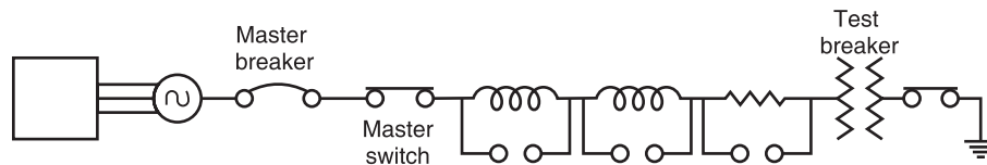
Fig. 5.4 Schematic diagram of a typical test plant
