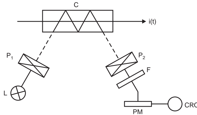
Fig. 4.30 Magneto-optical method
