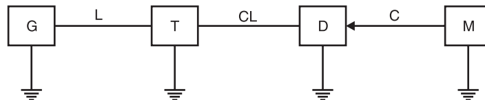
Fig. 4.17 Basic voltage testing circuit
