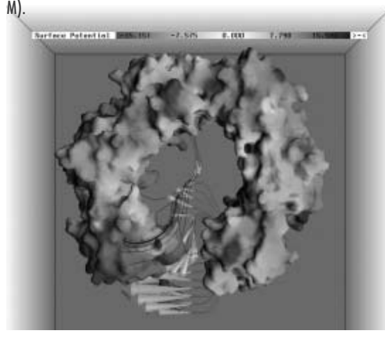
Colvin—Fig. 1. Electrostatic surface of the slightly opened \beta -clamp. Lines correspond to the lines of the electric field. Arrows indicate directionality of the electric field, and their size is proportional to the calculated force. Calculations were made in solution, considering dielectric constant 2.0 for the protein interior and 80.0 for the solvent and the physiological ionic strength (0.15 M).
