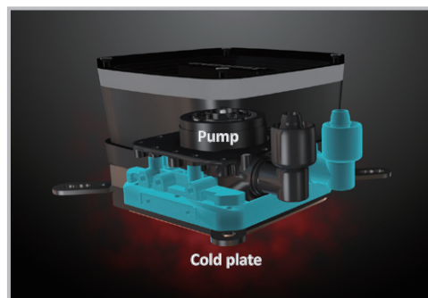
Dual Chamber water block design (patented)
