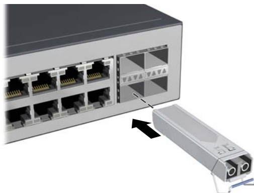
Figure 2-11. Installing an SFP transceiver
