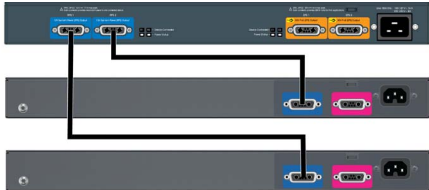
Figure 2-16. Connecting RPS to two switches
