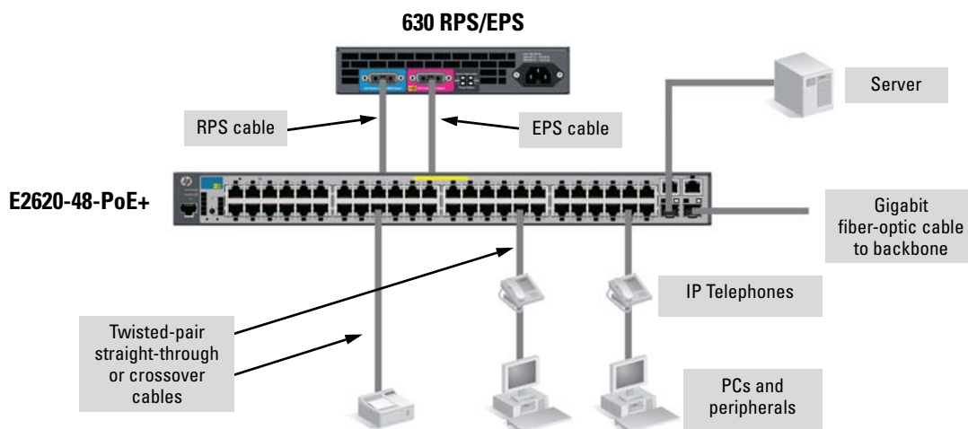
Figure 2-23. Basic desktop configuration with external power
