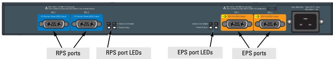
Figure 2-13. Back of the 620 RPS/EPS
