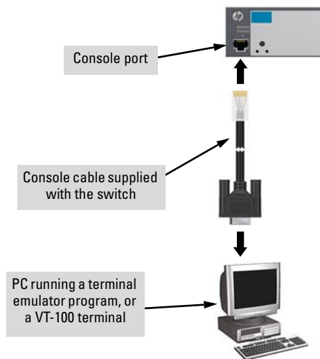
Figure 2-19. Connecting the console cable
