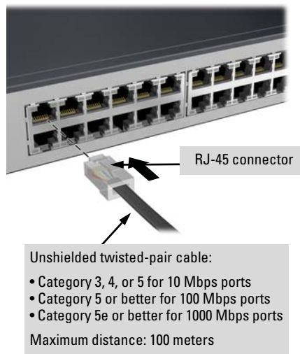
Figure 2-10. Connecting network cables
