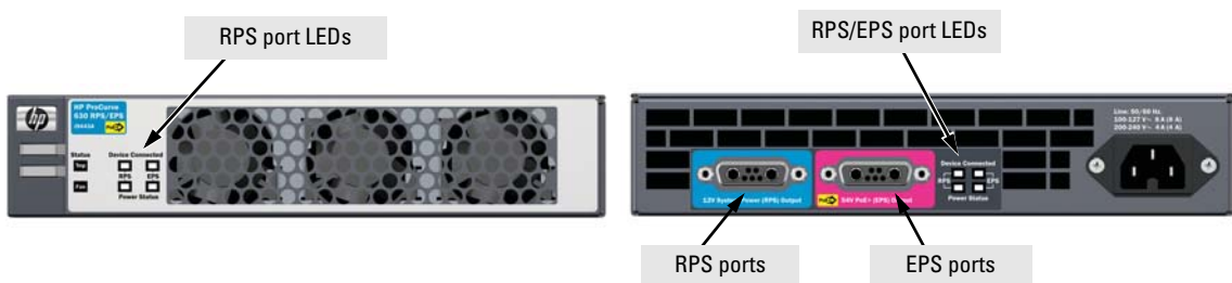
Figure 2-14. Front and back of the 630 RPS/EPS
