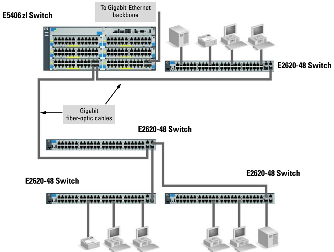
Figure 2-22. Networking to a gigabit ethernet backbone
