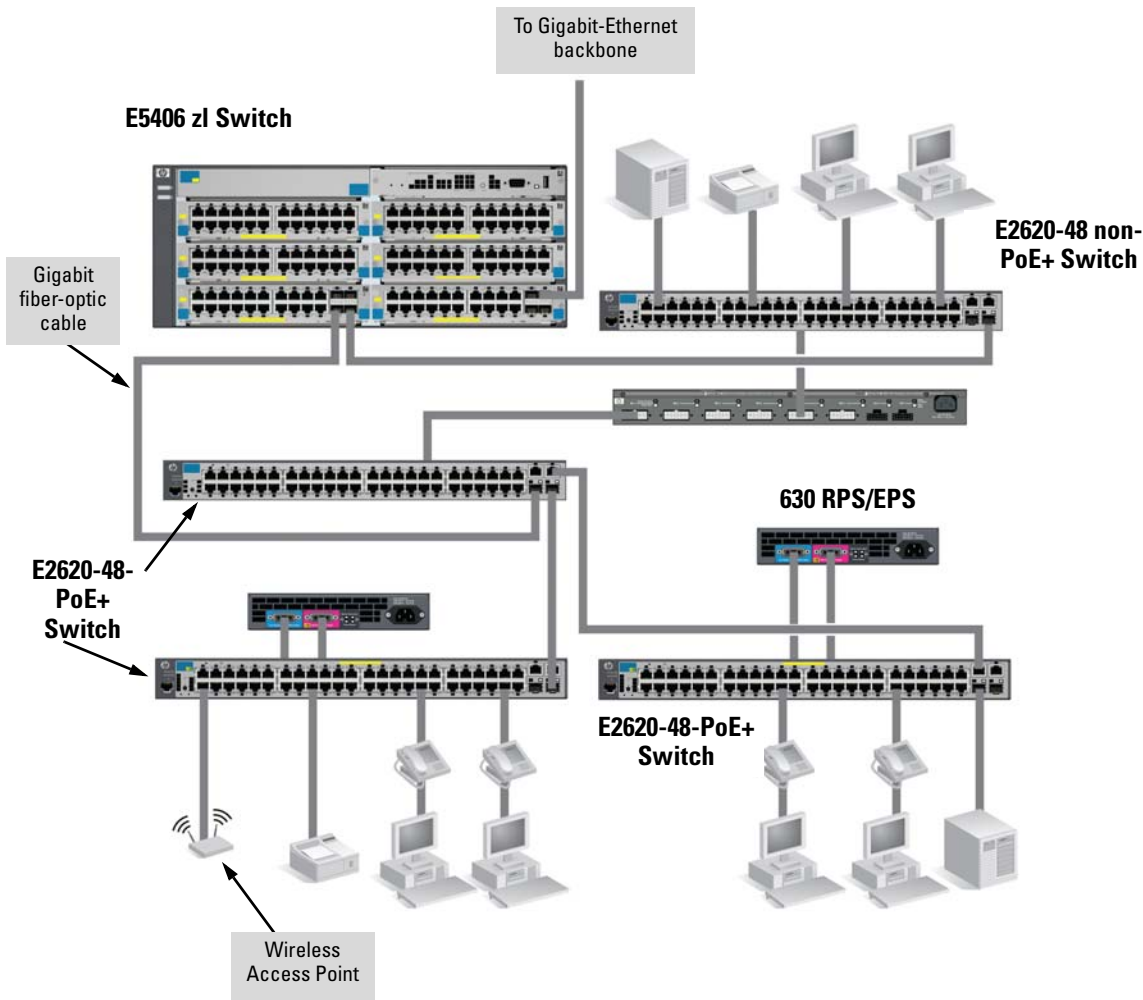
Figure 2-25. Networking PoE+ switches to a gigabit ethernet backbone
