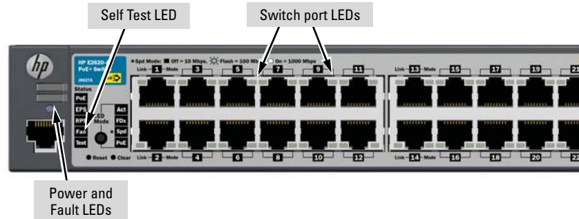
Figure 2-4. Checking the LEDs on the E2620-PoE+ switches
