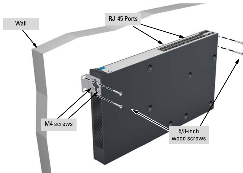
Figure 2-9. Wall mounting RJ-45 ports facing up
