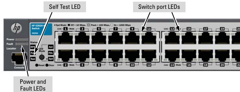
Figure 2-3. Checking the LEDs on the E2620 non-PoE+ switches
