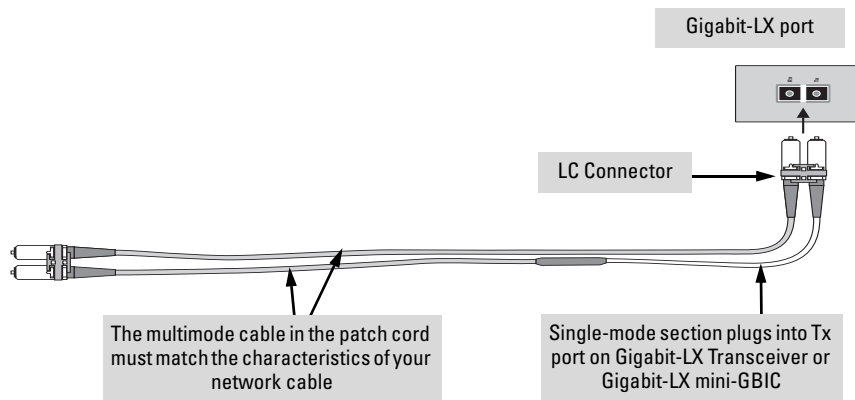
Figure B-1. Connecting a patch cord
