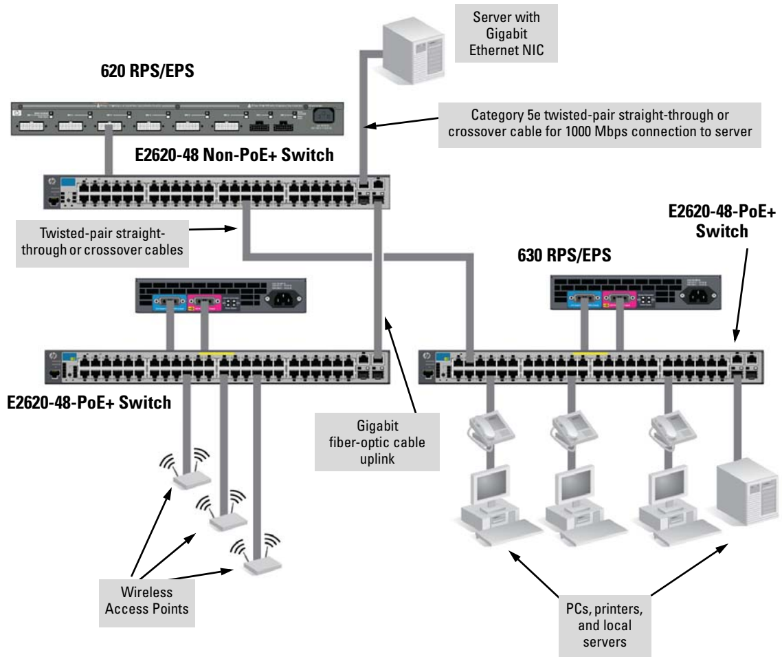
Figure 2-24. Segment network configuration with PoE+ switches
