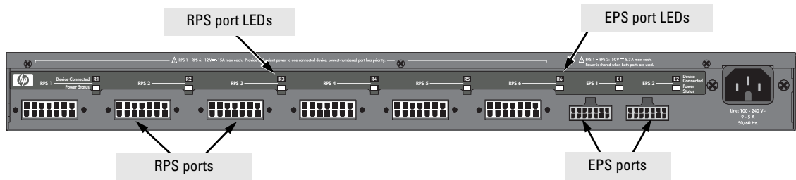
Figure 2-12. Back of the 600 RPS/EPS
