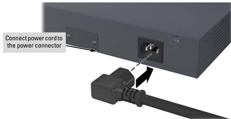
Figure 2-2. Example of connecting the power cord
