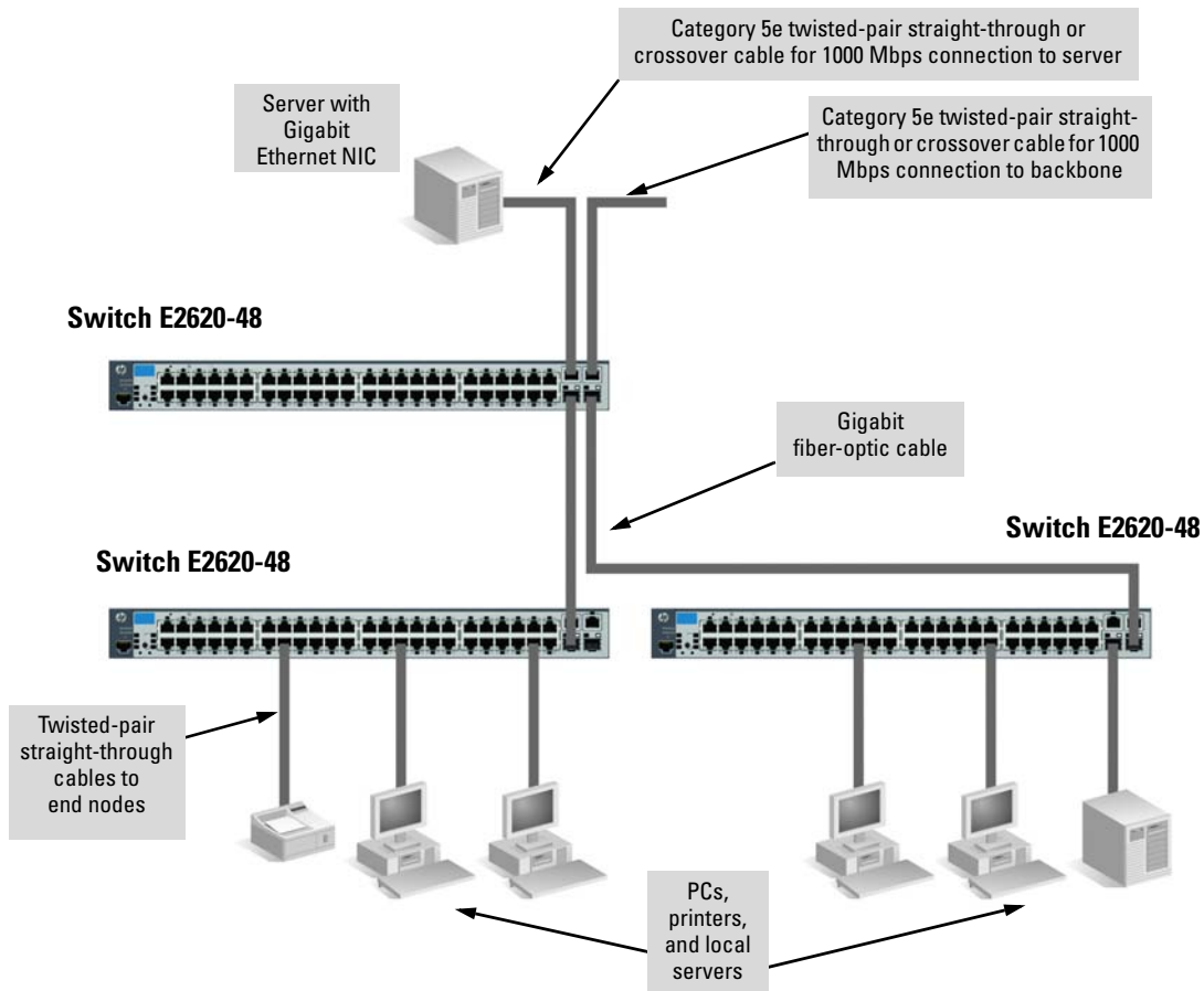
Figure 2-21. Segment network configuration
