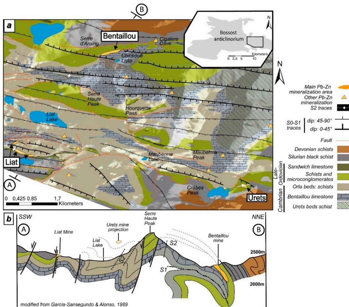
Figure 3. (a) Structural map of the Bentaillou-Liat-Urets district based on field study and BRGM/IGME geological maps. Location in Bossòst anticlinorium is indicated in the small sketch map (see also location on Figure 2a); (b) Structural NNE-SSW cross-section of the Liat-Bentaillou area. Location of the cross-section is indicated in the Figure 3a (modified from Garcia-Sansegundo and Alonso [56]). Note presence of Pb-Zn mineralization at rock competence interface and close to F1 fold hinge in Bentaillou mine.
