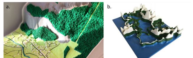
Figure 12: One solution to overcome the lack of colour in 3D printing is fabricating the physicalization in discrete pieces, each with a different filament colour, and assemble them. Image (a) taken from [ADMAS18] and image (b) taken from [TLI6].
