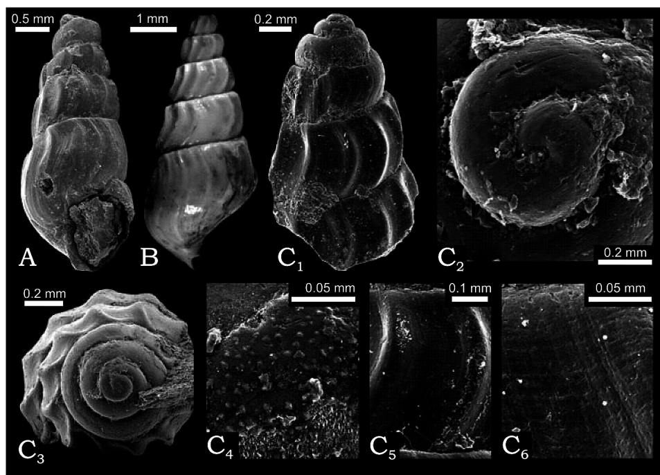
Fig. 11. Hudlestoniella undulata (Tullberg, 1881) from Timan region and Novaja Zemlja Island, Late Jurassic. A. ZPAL Ga.10/26 from Sevierno-Timanskaja, borehole 7, Timan region, Russia; lateral view. B. Holotype of Tullberg (1881), NRM Mo.1182 from Skodde Bay, Novaja Zemlja Island, Russia (light photograph, specimen not coated); lateral view. C. ZPAL Ga.10/22 from Sevierno-Timanskaja, borehole 218, Timan region, Russia; C 1 lateral view, C 2 close-up of the initial whorl in apical view, C 3 apical view, C 4 details of protoconch ornamentation, C 5 details of teleoconch ornamentation, C 6 close-up of the pitted spirae ornamenting teleoconch.
