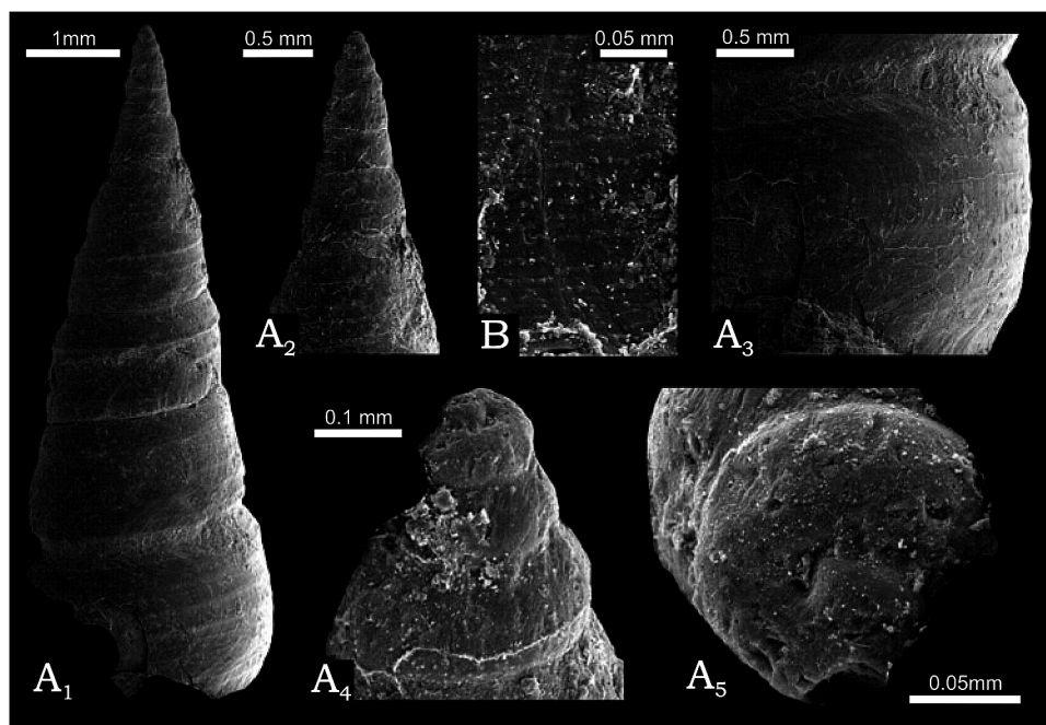
Fig. 5. Turritella turbinæ Beisel, 1991 from Krasnyj Agronom, borehole 16, Western Siberia, Maastrichtian (Late Cretaceous). A. ZPAL Ga.10/13; A 1 lateral view, A 2 apex in lateral view, A 3 details of the late teleoconch ornamentation, A 4 protoconch in lateral view, A 5 initial whorl in apical view. B. ZPAL Ga.10/14; details of the early teleoconch ornamentation.
