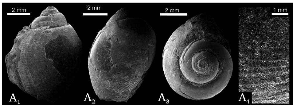
Fig. 8. Gen. et sp. indet. 2 from Yatrija River, Western Siberia, Russia, Early Valanginian (Early Cretaceous). ZPAL Ga.10/20; A 1 lateral view, A 2 lateral view, slightly oblique to show the base ornamentation, A 3 apical view, A 4 details of teleoconch ornamentation.
