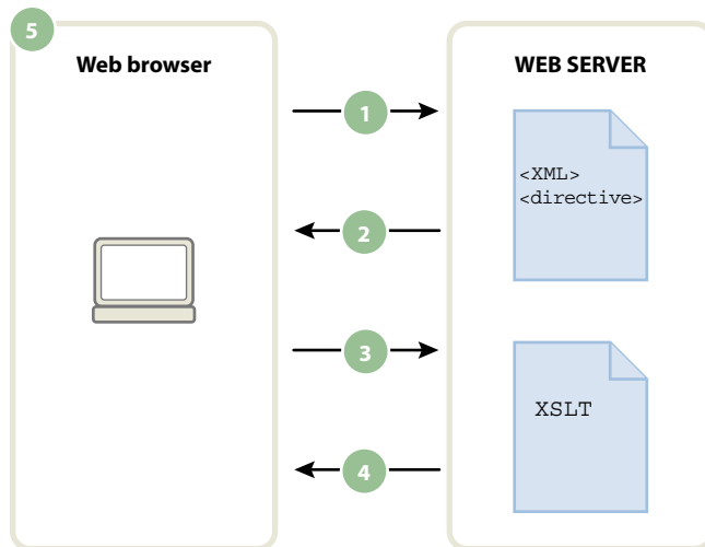
1. Browser requests XML file 2. Server responds by sending XML file to browser 3. Browser reads XML directive and calls XSLT file 4. Server sends XSLT file to browser 5. Browser transforms XML data and displays it in browser
