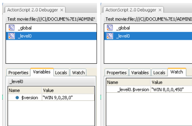
Variables marked for the Watch list and variables in the Watch list
