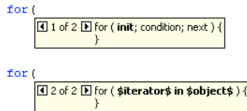
A code hint with multiple sets of parameters
