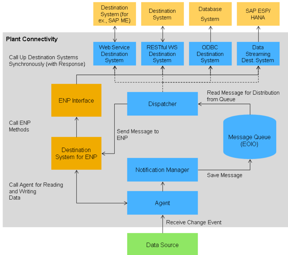
Notification Process with Enhanced Notification Processing (ENP)
