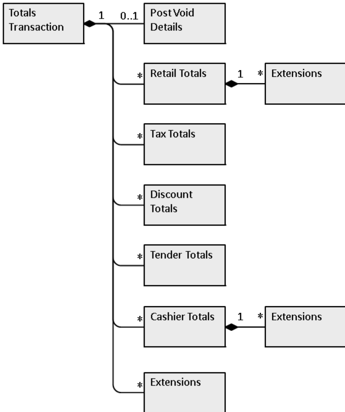
Structure of a Totals Transaction
