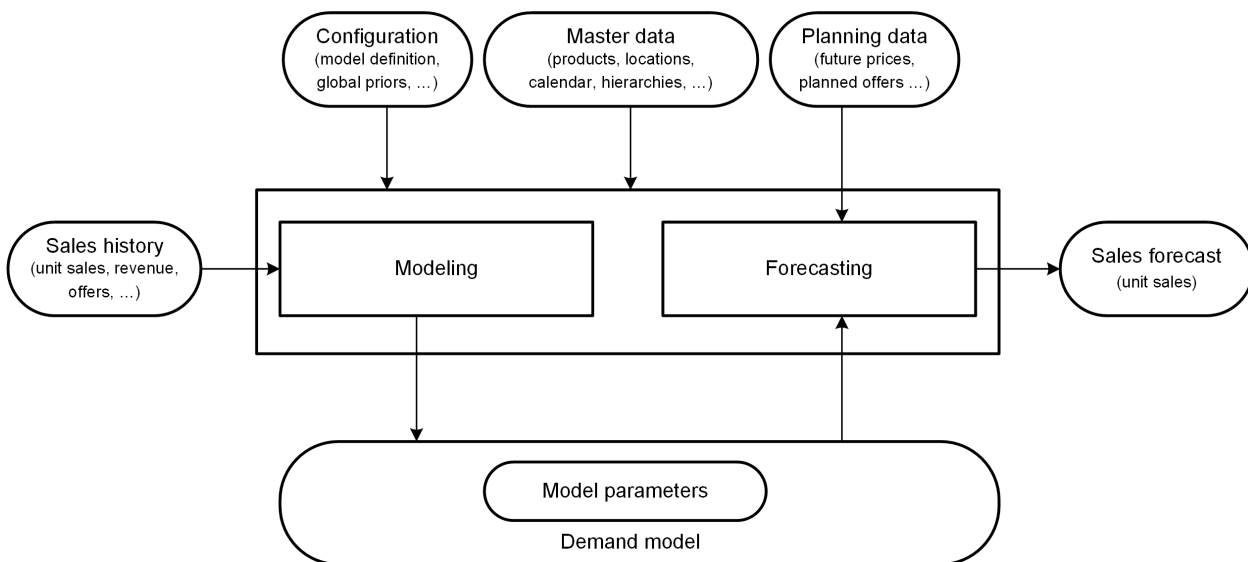
Data Flow in Modeling and Forecasting with UDF
