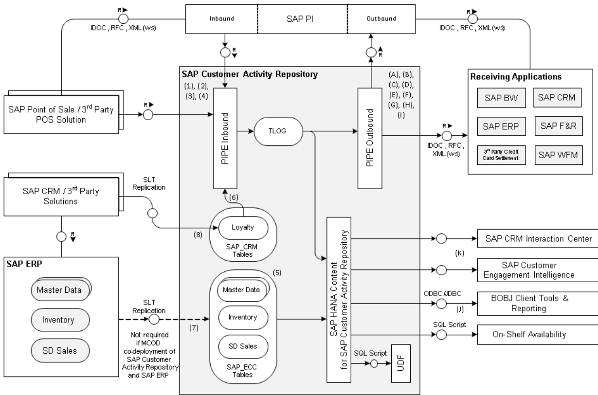
SAP Customer Activity Repository Data Flow Process
