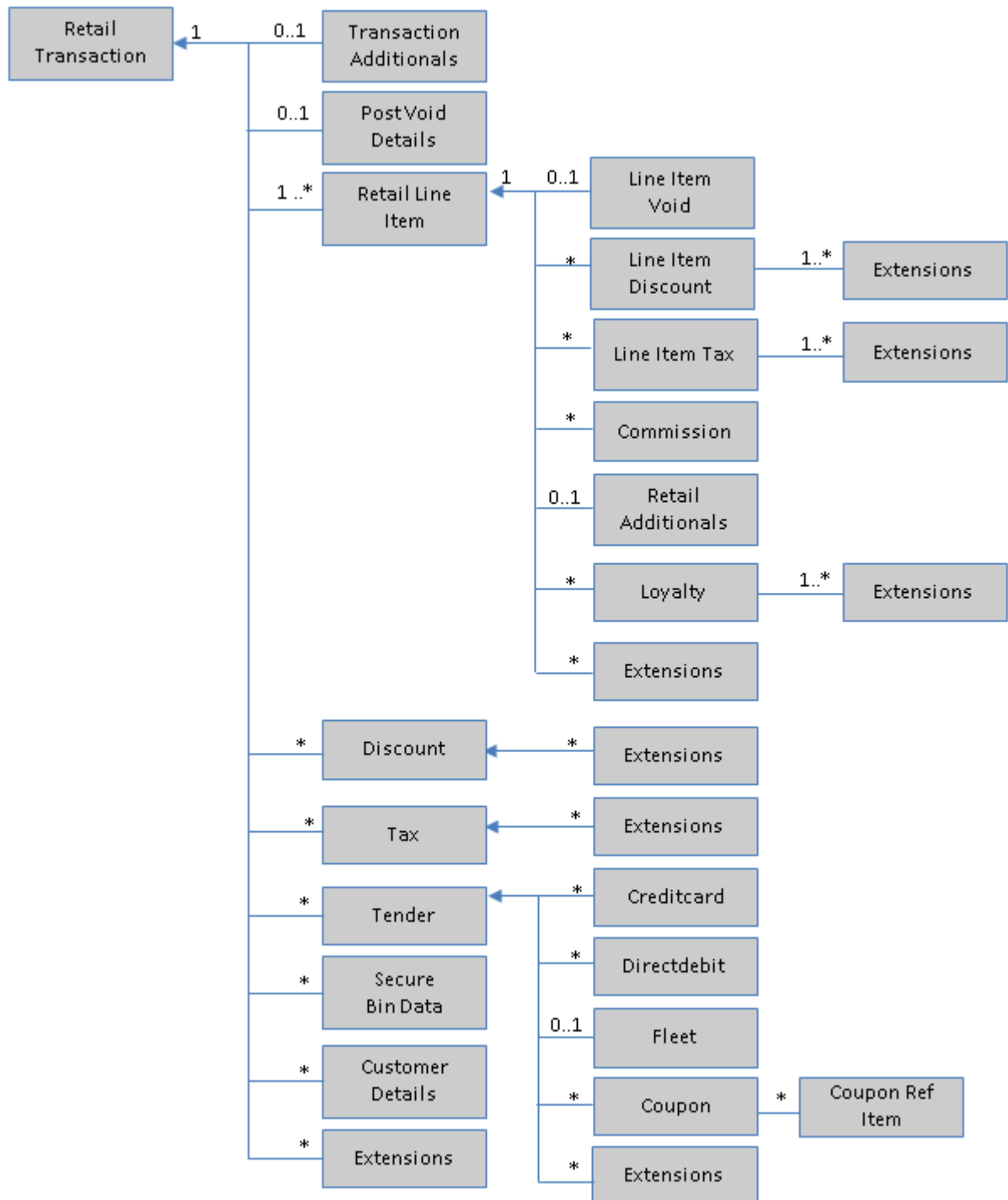
Structure of a Retail Transaction
