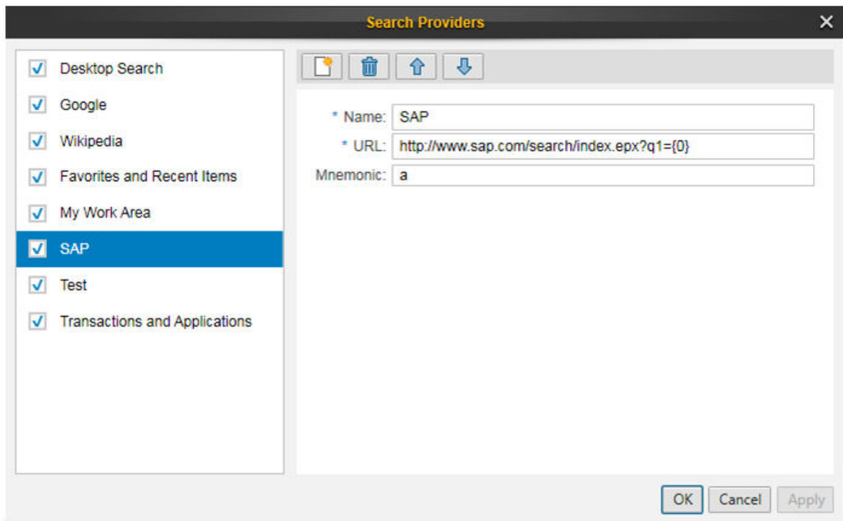
Example Search Providers Dialog Box
