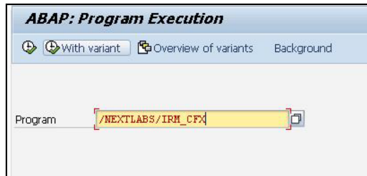
Figure 5-8: IRM_CFX Program
