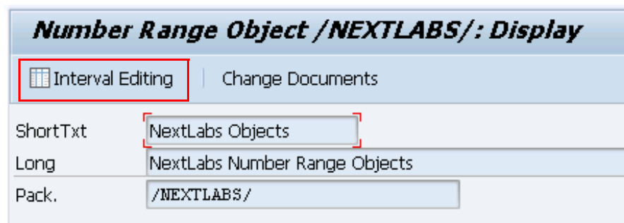
Figure 4-31: Number Ranges
