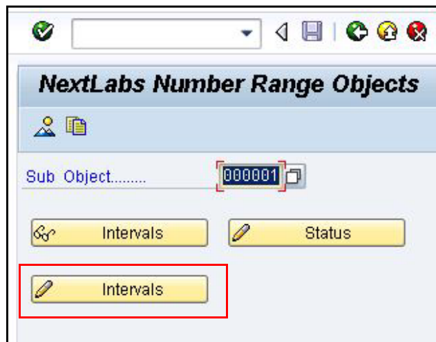
Figure 4-34: Changing Intervals
