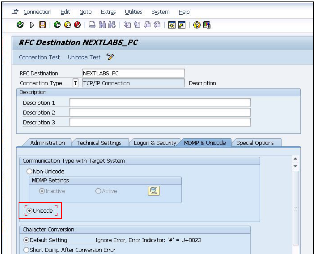
Figure 3-20: Selecting Unicode
