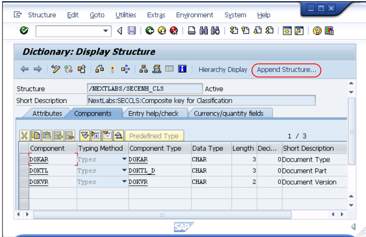
Figure 4-12: Append Structure
