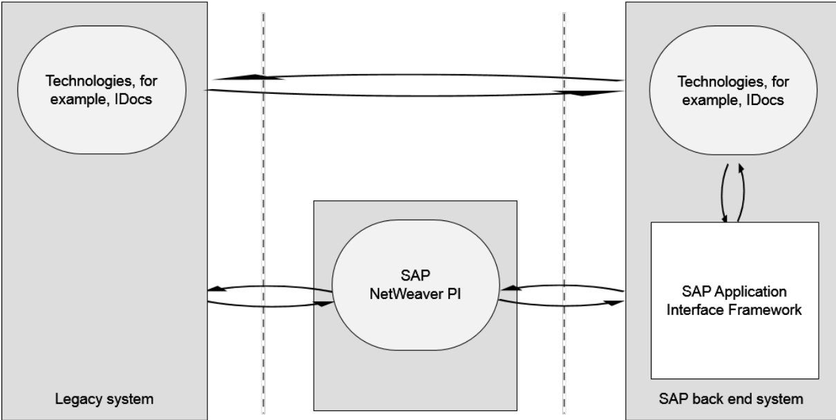
Figure 1: System Landscape
