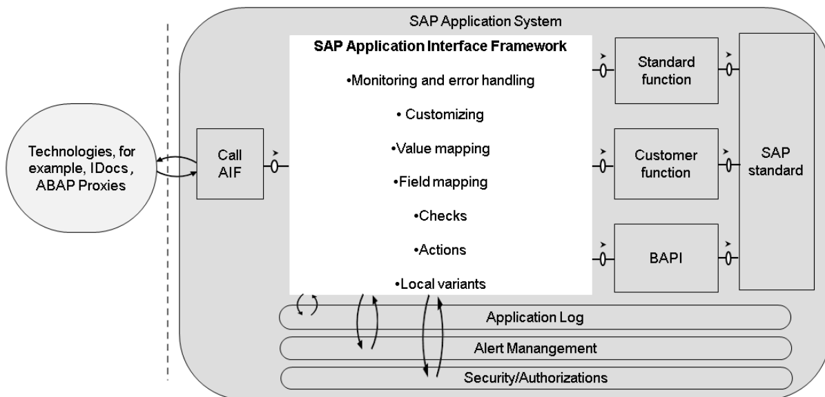
Figure 2: System Architecture
