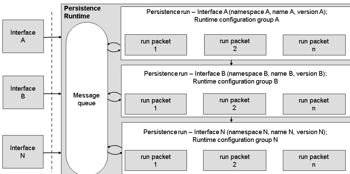
Figure 16: AIF Runtime
