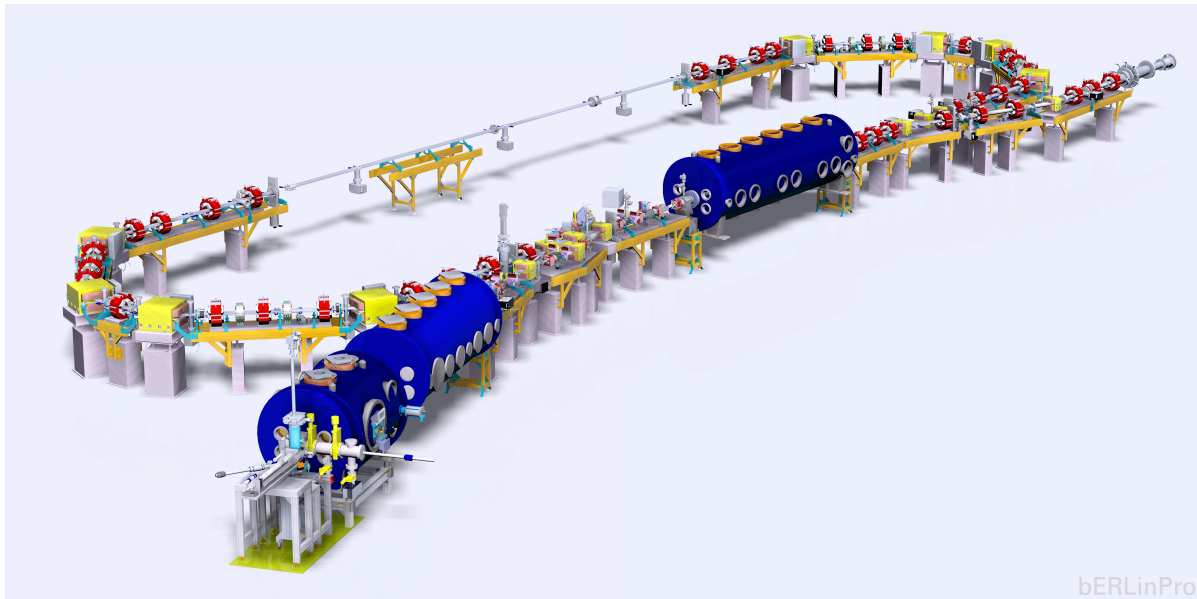
Figure 2.25.: Schematic of bERLinPro. From bottom left to top right: SRF photoinjector, booster module, merger, main linac module, and beam dump.
