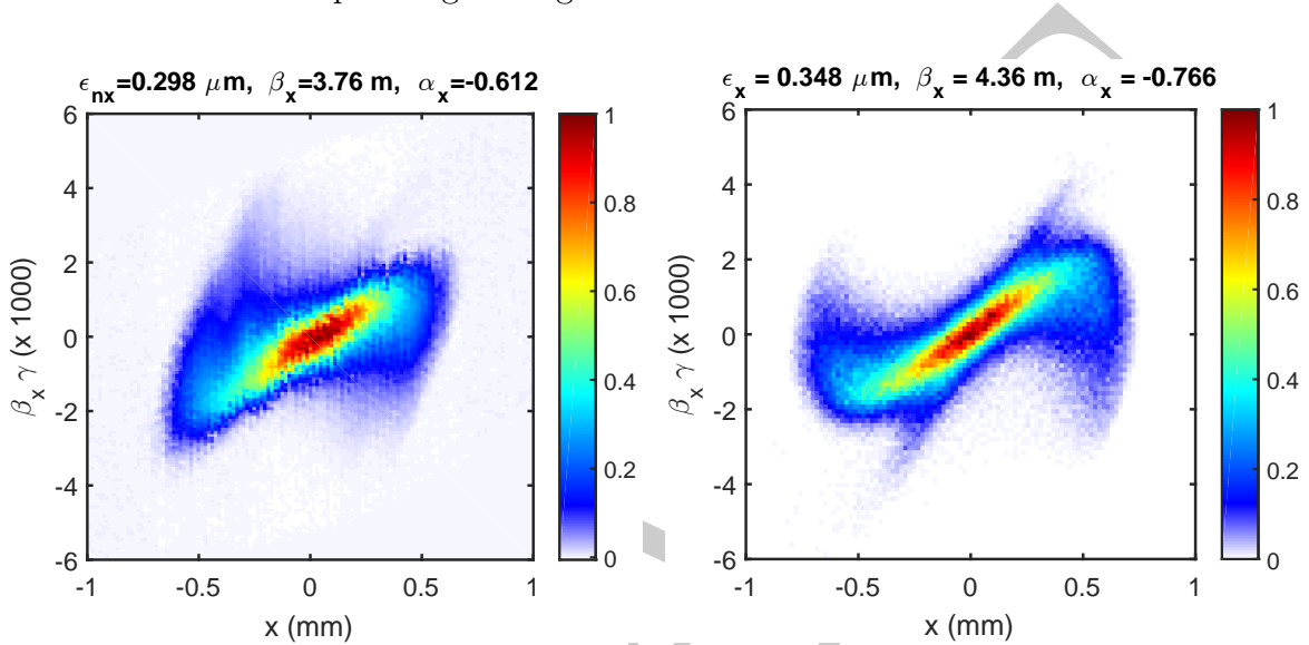
Figure 2.17.: Measured (left) and simulated (right) transverse phase spaces after the injector at 5 pC.
