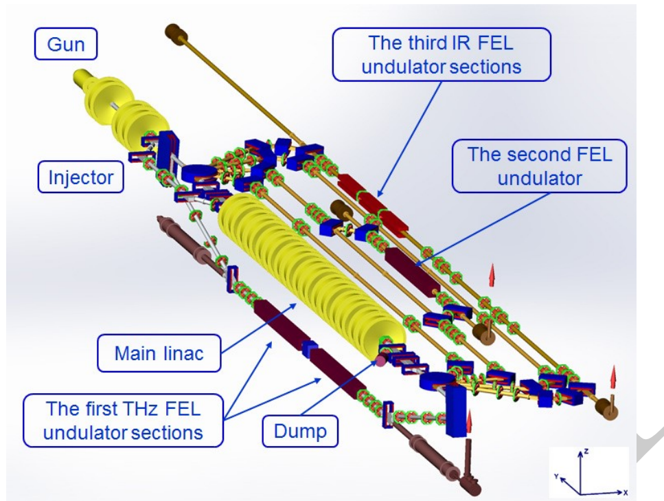
Figure 2.29.: The Novosibirsk ERL with three FELs (top view).
