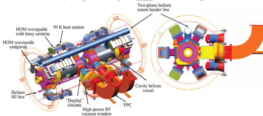
Figure 4.6.: Conceptual cryomodule design for high-current ERLs with a JLab HC cavity pair (figure taken from [180]). Each cavity employs six HOM waveguide dampers with one doing double duty as an FPC.
