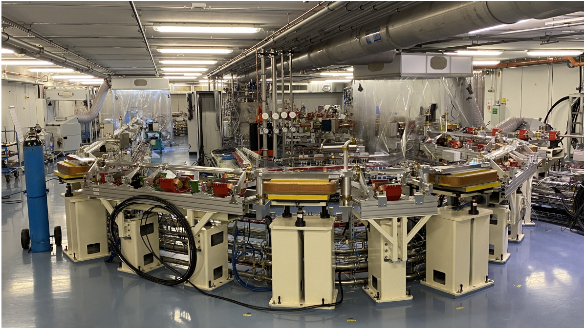
Figure 2.26.: bERLinPro during the installation of the recirculator vacuum system under clean room conditions. The magnets of the return arc are open for the installation. The injection line comes from the right.
