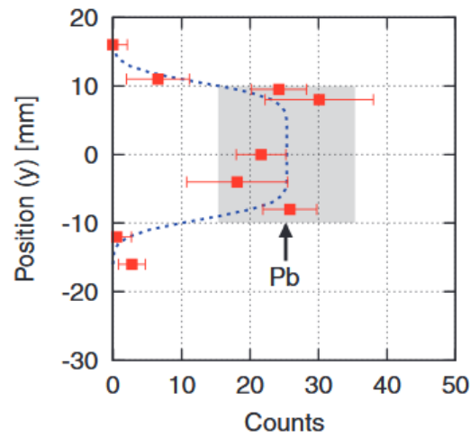
Figure 5.20.: Counts detected as a function of vertical gamma beam position during a scan of a small lead block. From Ref. [337].
