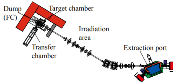
Figure 2.28.: Layout of the irradiation area.
