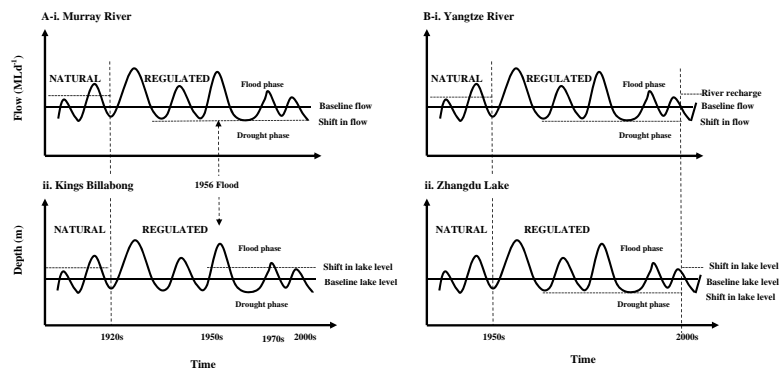
Figure 3. Hydrological frameworks of Murray and Yangtze rivers. (ai, aii): River Murray: regulation was imposed by humans in the 1920s, which resulted in low water volume in the downstream river channels, but Kings Billabong was converted to a water storage tank permanently led to higher lake level, subsequently ceased natural dry-wet cycles; (bi, bii): Yangtze River: the first large scale human impact on the river was imposed during the c. 1950s, which ceased naturally occurring flood pulses in adjacent wetlands leading to a drying up of the river channel connecting to wetlands including low water volume in Zhangdu Lake.
