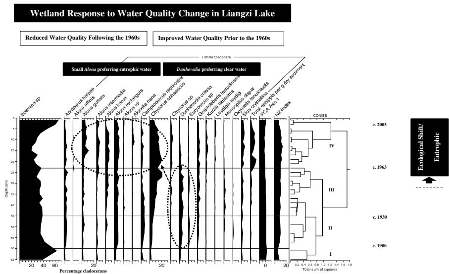
Figure 6. Composition (%) and N2 diversity index of subfossil cladocedans in Liangzi Lake, and their response to past water quality change.
