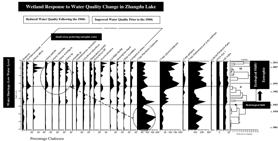
Figure 5. Composition (%) and N2 diversity index of subfossil cladocedans in Zhangdu Lake, and their response to past hydrological and water quality change.
