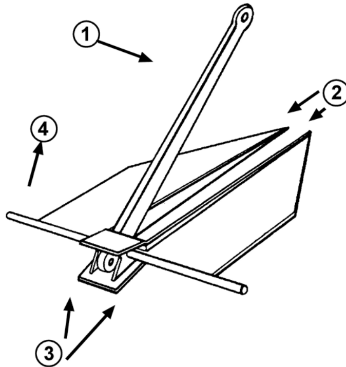
Figure 6-32 Main Parts of a Danforth Anchor
