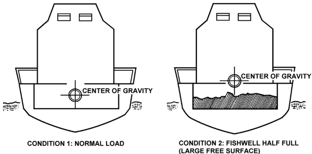
Figure 4-4 Effects of Free Surface
