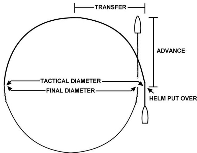
Figure 6-20 Turning Characteristics
