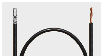
Wire end ferrule 2.8 : open. Cable 300 mm. Cable type 3
