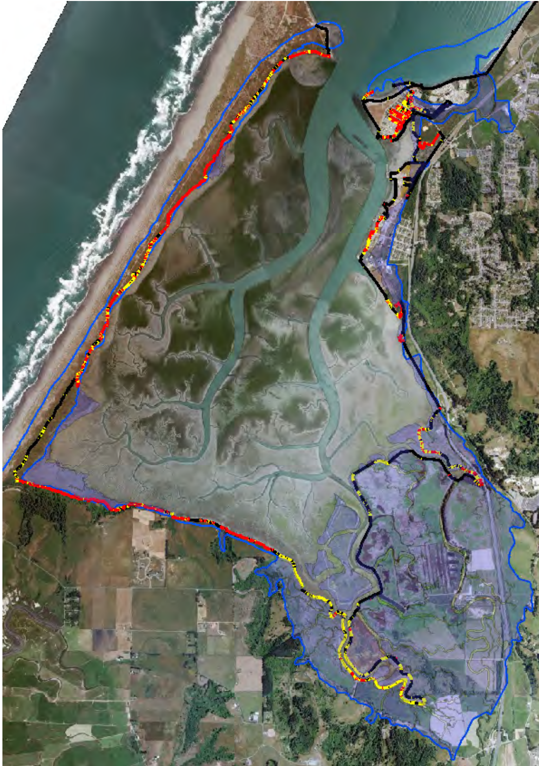
Figure 81. South Bay, shoreline areas overtopped by 1 foot of sea level rise (red), and 2 feet (yellow), and the 1870 tidal inundation footprint (blue).
