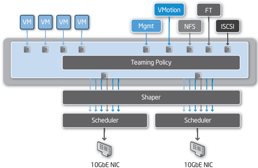
Figure 9. The NetIOC software-based scheduler manages bandwidth resources among various types of traffic.
