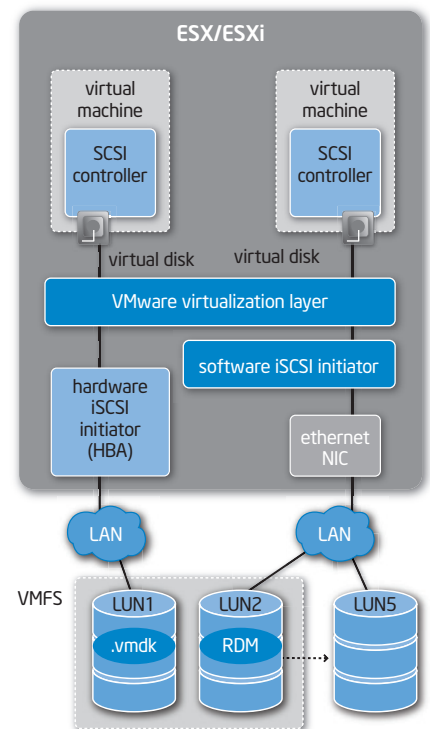
Figure 7. Native software-based iSCSI adapter/initiators and dependent hardware iSCSI adapters are examples of adapters ESX uses to provide iSCSI connections.
