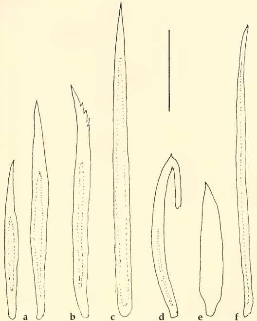
Fig. 3. Eleutheromenia carinata , spec. nov. (Solenogastres): mantle sclerites (see text); bar = 50 \mu\text{m} .
