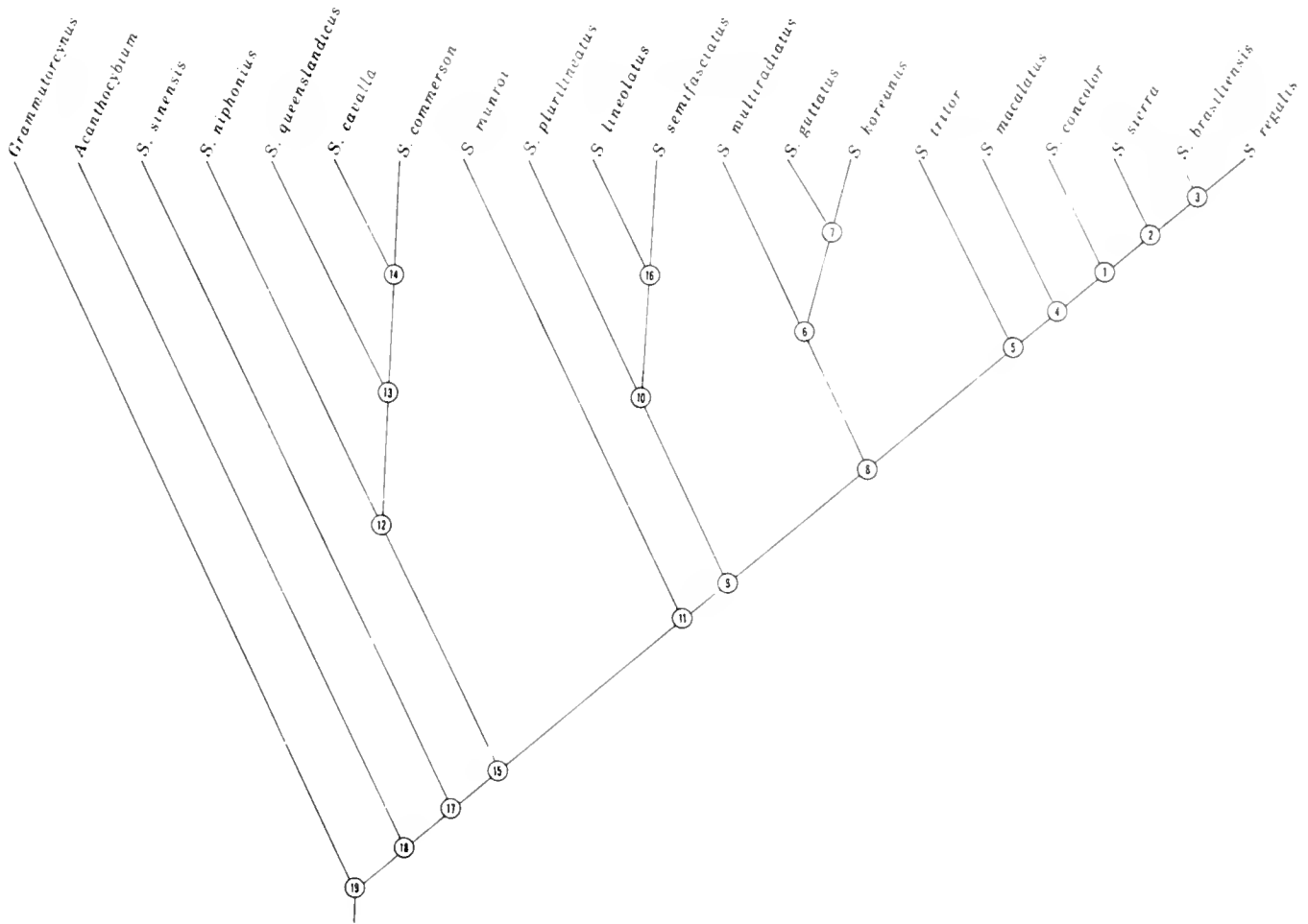
Fig. 325. Cladogram of relationships within the Scomberomorini (from Collette and Russo, in press).
