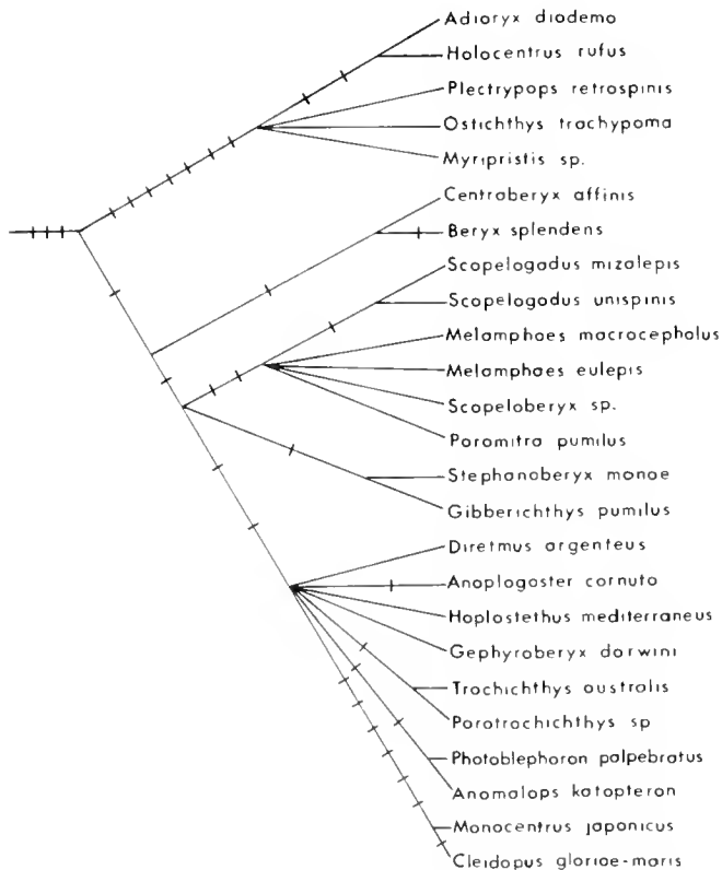
Fig. 211. Cladogram showing the relationships of the beryciform families studied by Zehren (1979).
