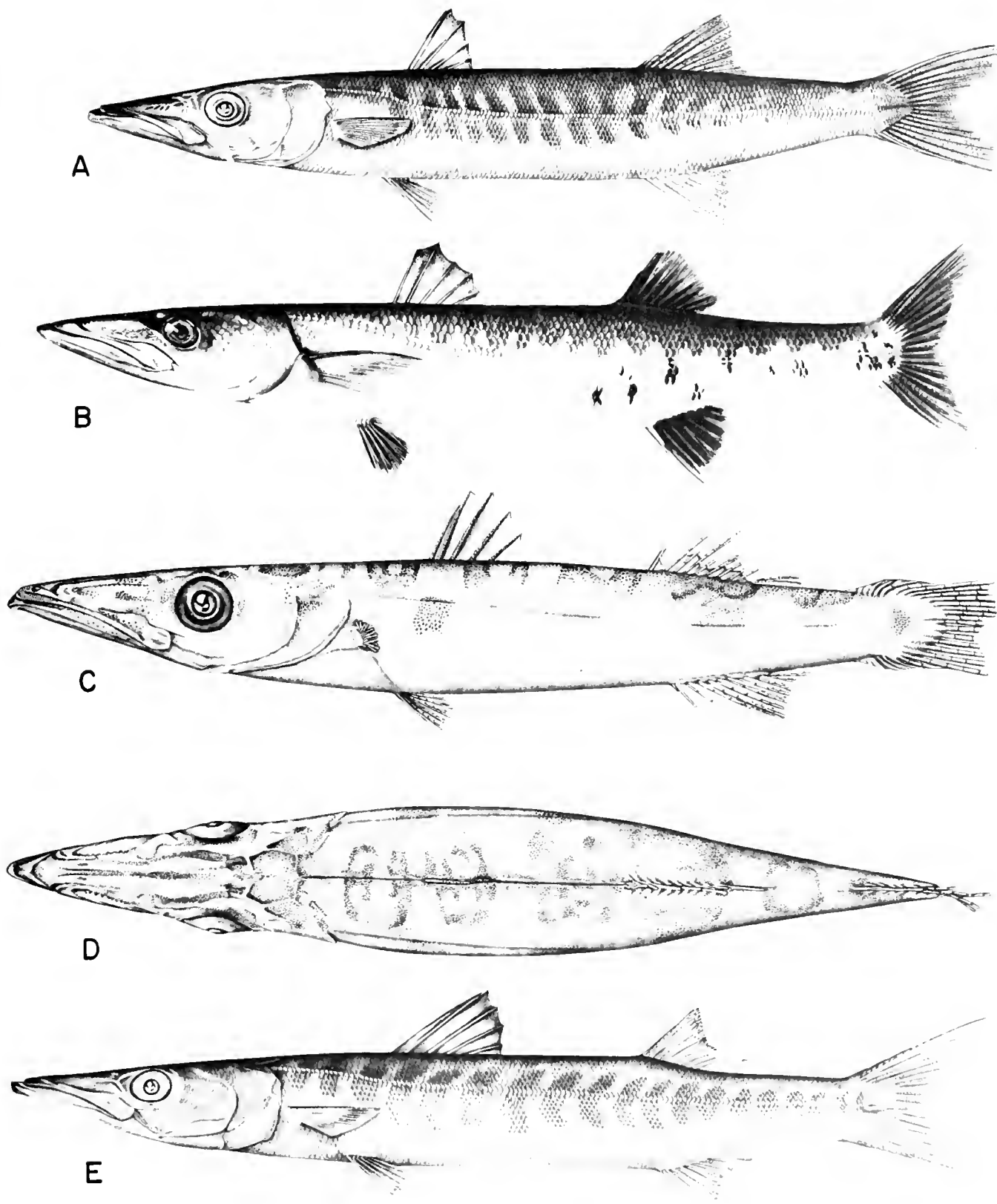
Fig. 289. Variation in pigmentation in various species of Sphyraena . (A) Sphyraena gene , 29 cm, Makassar, Indonesia; (B) Sphyraena barracuda , 63 cm, Biscayne Bay, Miami, Florida; (C) Sphyraena forsteri , 5.9 cm, Indonesia, lateral view; (D) Sphyraena forsteri , 5.9 cm, Indonesia, dorsal view; and (E) Sphyraena putnami , 45.7 cm, Mahé, Seychelles Islands. (All drawn by J. I. Godfrey.)
