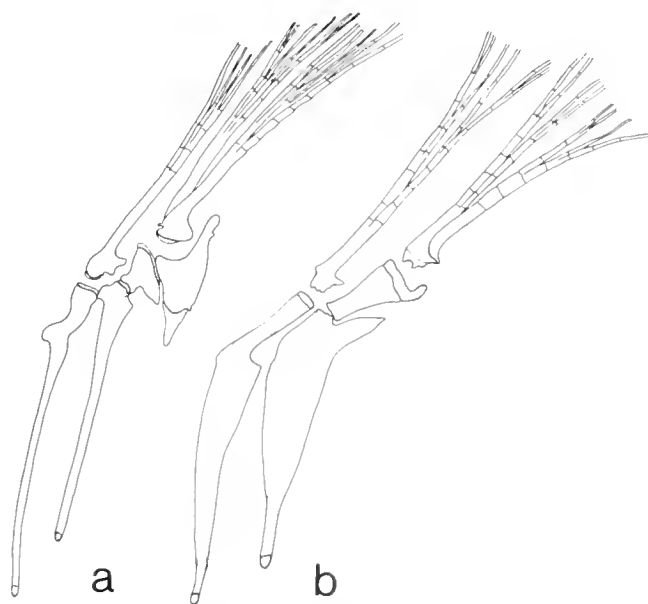
Fig. 277. Terminal pair of dorsal fin rays and associated pterygiophores: (a) Nematistius pectoralis (Note presence of large bony stay behind last medial pterygiophore) and (b) Naucrates ductor .
