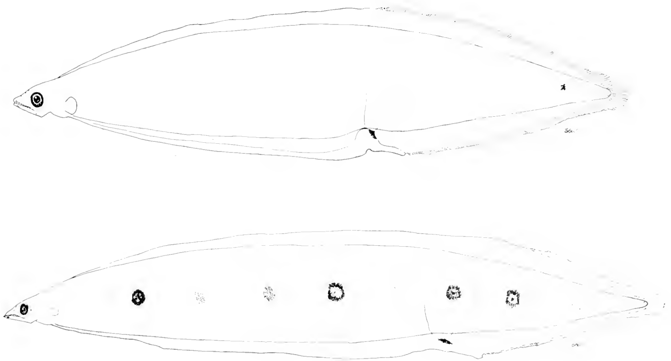
Fig. 45. Leptocephali of Neoconger (above) and Moringua (below) (Moringuidae).
