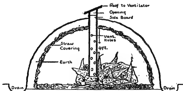
FIG. 64.—Diagram of a vegetable pit. It should run east and west and the mouth of the ventilator should slant north. Have eight inches of straw at the base of the pit. As the weather grows colder add more earth, as indicated, to keep out the frost.
