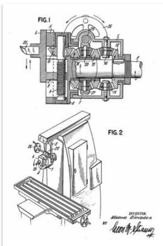
Device to Impart Radial Displacements to Eccentrically Rotating Parts, in «United States Patent Office», 1 marzo 1960.
