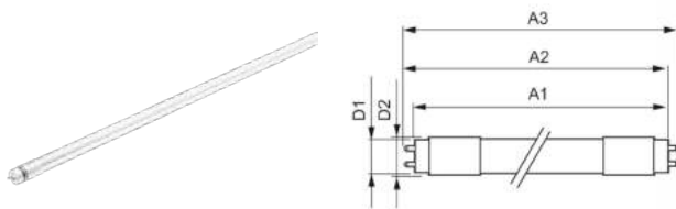
CorePro LEDtube HF 600mm
