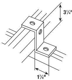
CZ209 For attaching "A" back to back.
