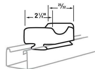
AB-880 AB-881 3" and 4" Porcelain Saddles
