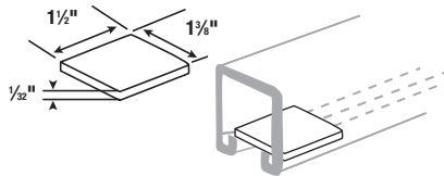
AB868 Fiber Retainer for cables until closure strip is installed.
