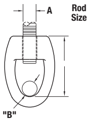
M-117 MI Socket only for S Split Ring Hanger Sizes ⅝" through ⅞" Rod Federal Type 16 SP69 Type 16
