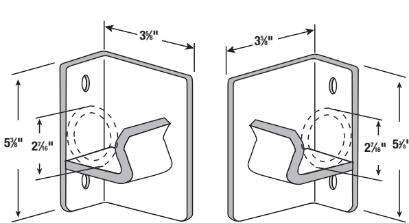
Q255 For 2" standard pipe. Load 1,500 lbs.
