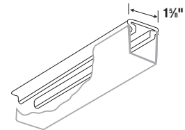
AB-844* Steel Closure Strip AB-844-PC* Plastic Closure Strip When used as a raceway channel, it is normally installed with the slot up and after wiring is complete, the closure strip is installed. For all channels. Standard lengths 10 ft.
