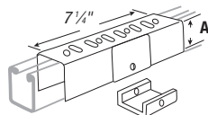
822 Raceway Joiner & Seal
