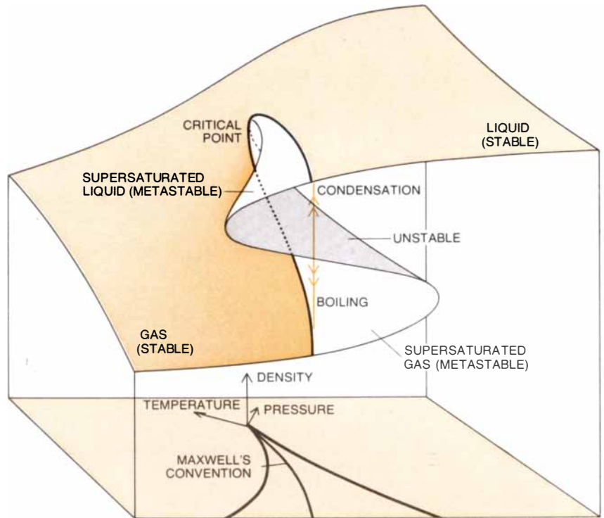
PHASE TRANSITIONS between the liquid and the gaseous state of matter conform to a modified cusp model in which temperature and pressure are the control factors. Ordinarily both boiling and condensation take place at the same values of temperature and pressure. Thus there are catastrophic changes, but there is no hysteresis. Under special circumstances, however, a vapor can be cooled below its dew point and a liquid can be heated above its boiling point, so that the behavior surface is followed all the way to the fold curve. The critical point, where liquid and gas exist simultaneously, is represented by the singularity where the pleat disappears.
