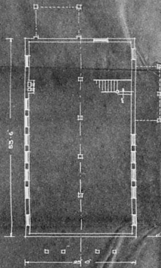
BASEMENT PLAN
